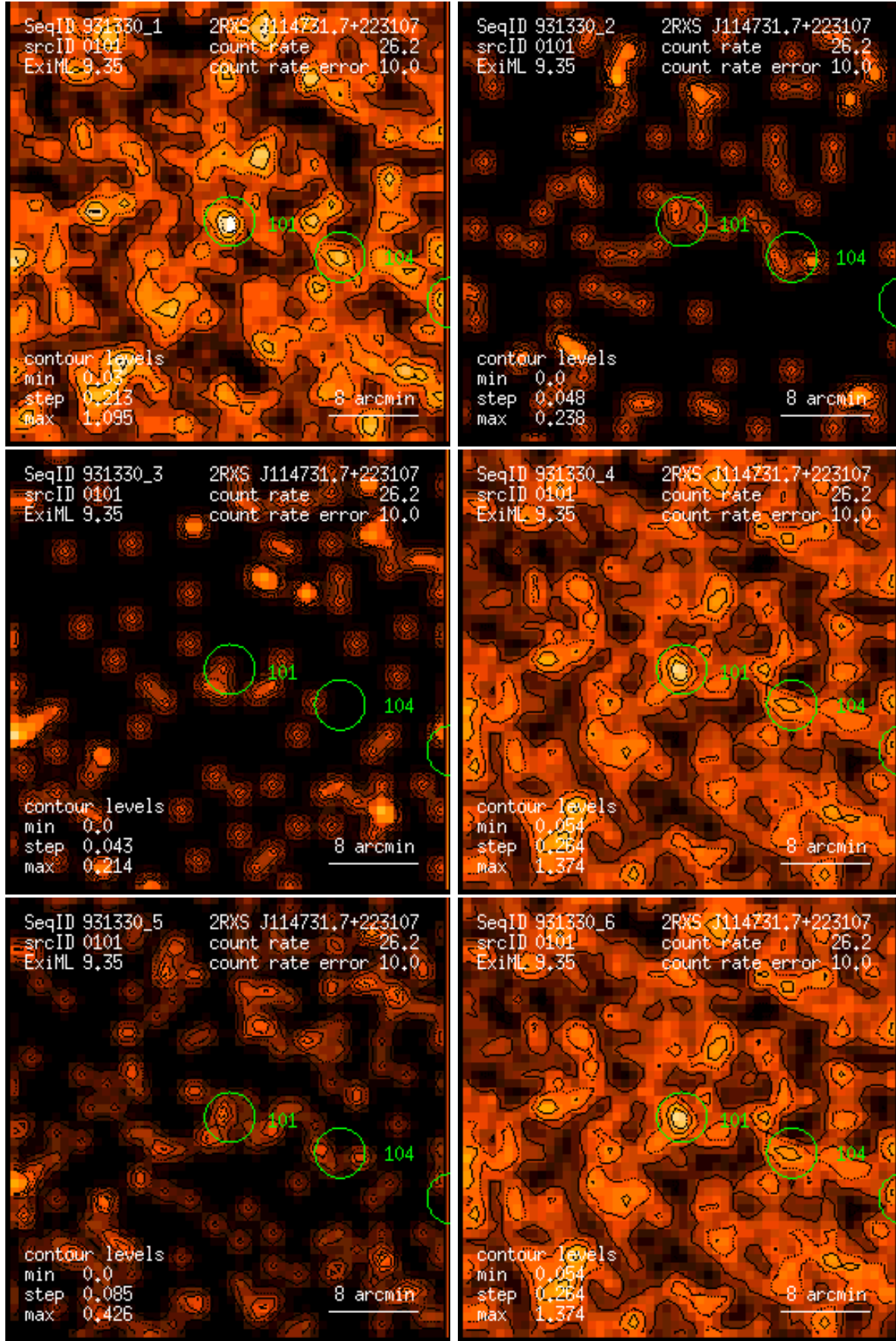
Figure 101: RASS 931330: detection 0101: band rate images, Gaussian filter: (1) PSPC channels 11 – 41, (2) 52 – 90, (3) 91 – 201, (4) 11 – 235, (5) 52 – 201, (6) 11 – 201. Broad band rates in counts/ks. Band rate contour levels in counts/ks/arcmin 2 .
