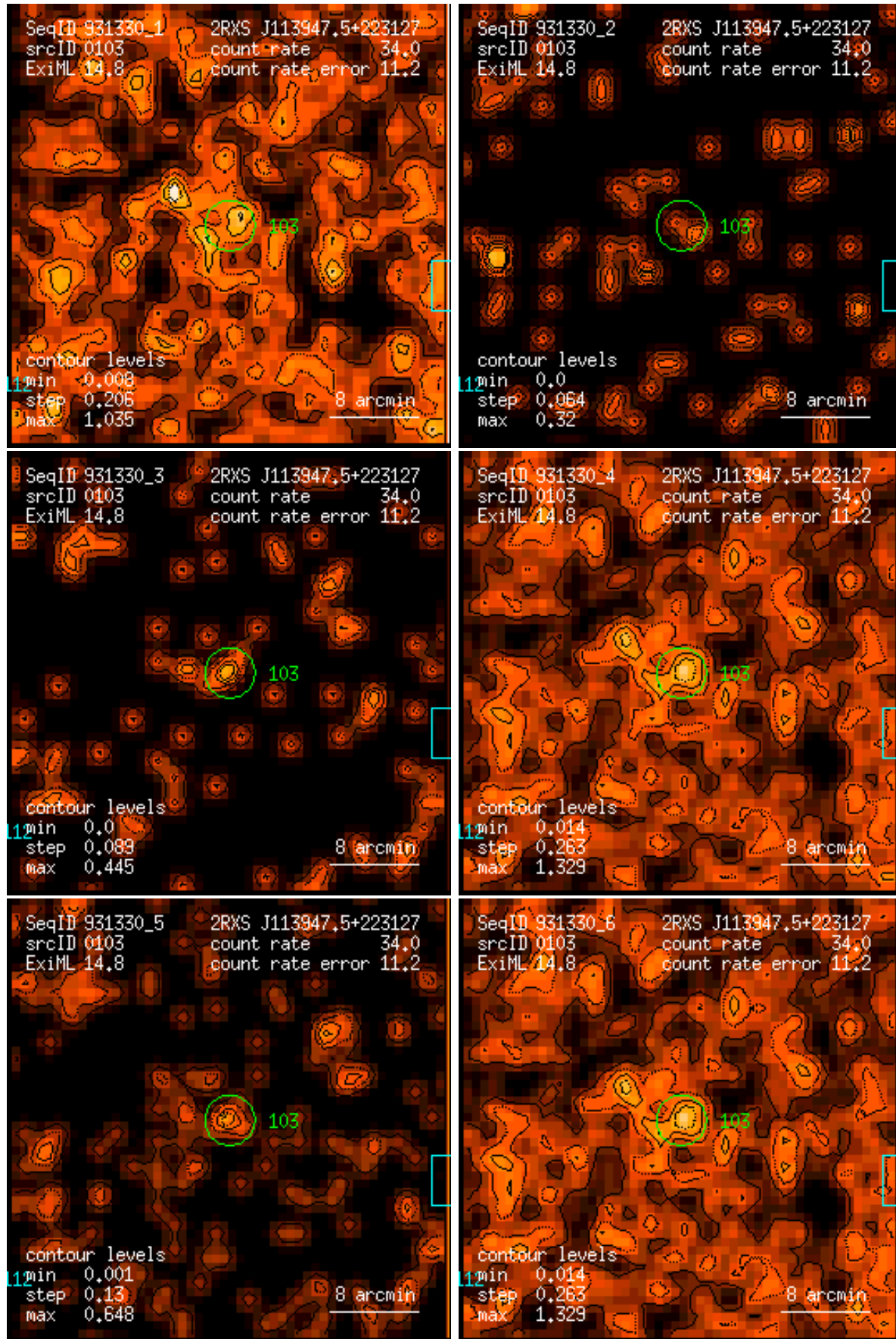
Figure 103: RASS 931330: detection 0103: band rate images, Gaussian filter: (1) PSPC channels 11 – 41, (2) 52 – 90, (3) 91 – 201, (4) 11 – 235, (5) 52 – 201, (6) 11 – 201. Broad band rates in counts/ks. Band rate contour levels in counts/ks/arcmin 2 .
