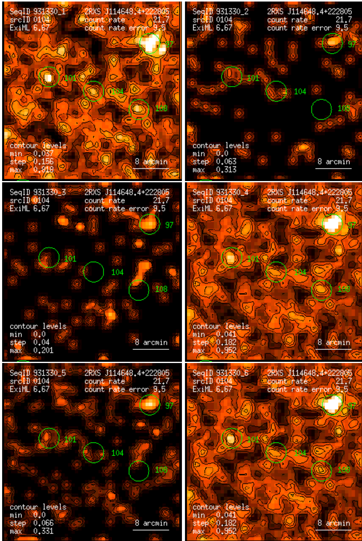
Figure 104: RASS 931330: detection 0104: band rate images, Gaussian filter: (1) PSPC channels 11 – 41, (2) 52 – 90, (3) 91 – 201, (4) 11 – 235, (5) 52 – 201, (6) 11 – 201. Broad band rates in counts/ks. Band rate contour levels in counts/ks/arcmin 2 .
