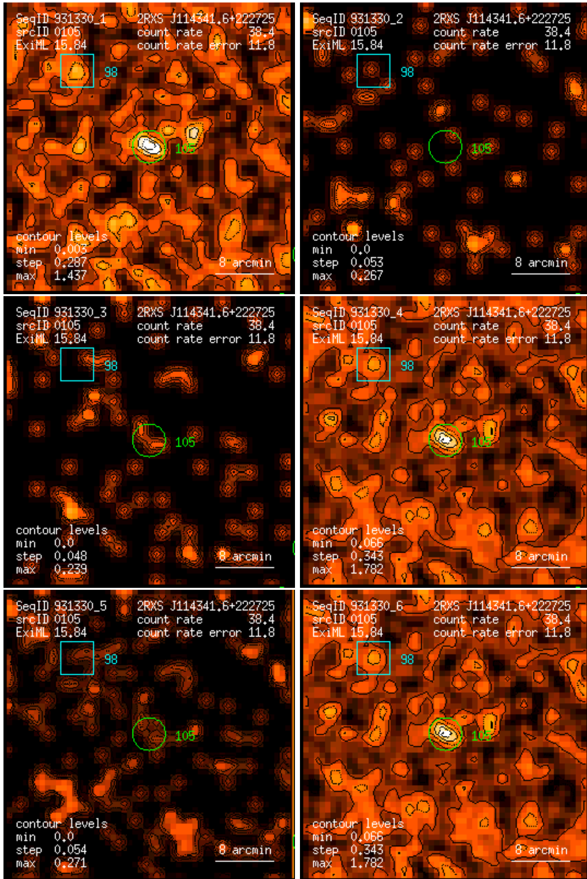
Figure 105: RASS 931330: detection 0105: band rate images, Gaussian filter: (1) PSPC channels 11 – 41, (2) 52 – 90, (3) 91 – 201, (4) 11 – 235, (5) 52 – 201, (6) 11 – 201. Broad band rates in counts/ks. Band rate contour levels in counts/ks/arcmin 2 .
