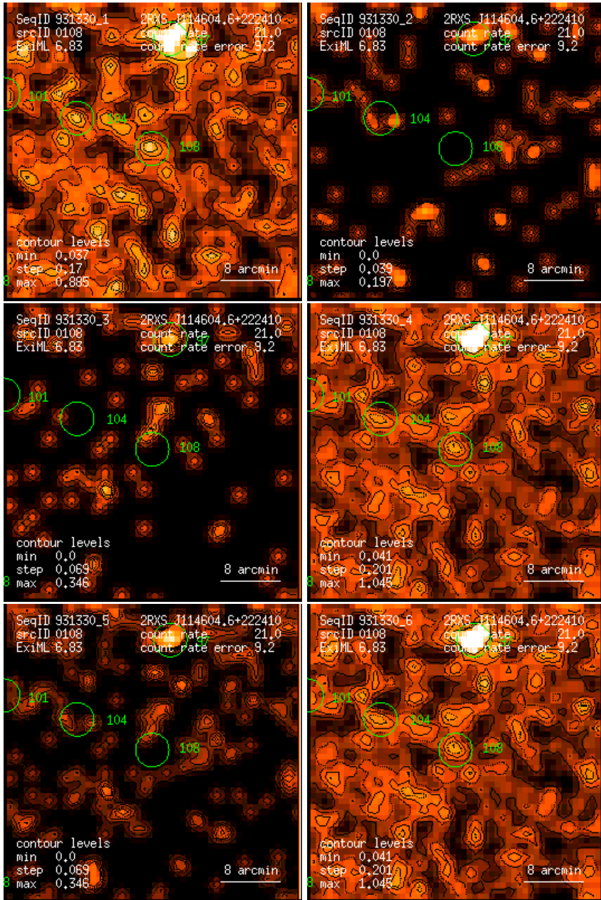
Figure 108: RASS 931330: detection 0108: band rate images, Gaussian filter: (1) PSPC channels 11 – 41, (2) 52 – 90, (3) 91 – 201, (4) 11 – 235, (5) 52 – 201, (6) 11 – 201. Broad band rates in counts/ks. Band rate contour levels in counts/ks/arcmin 2 .
