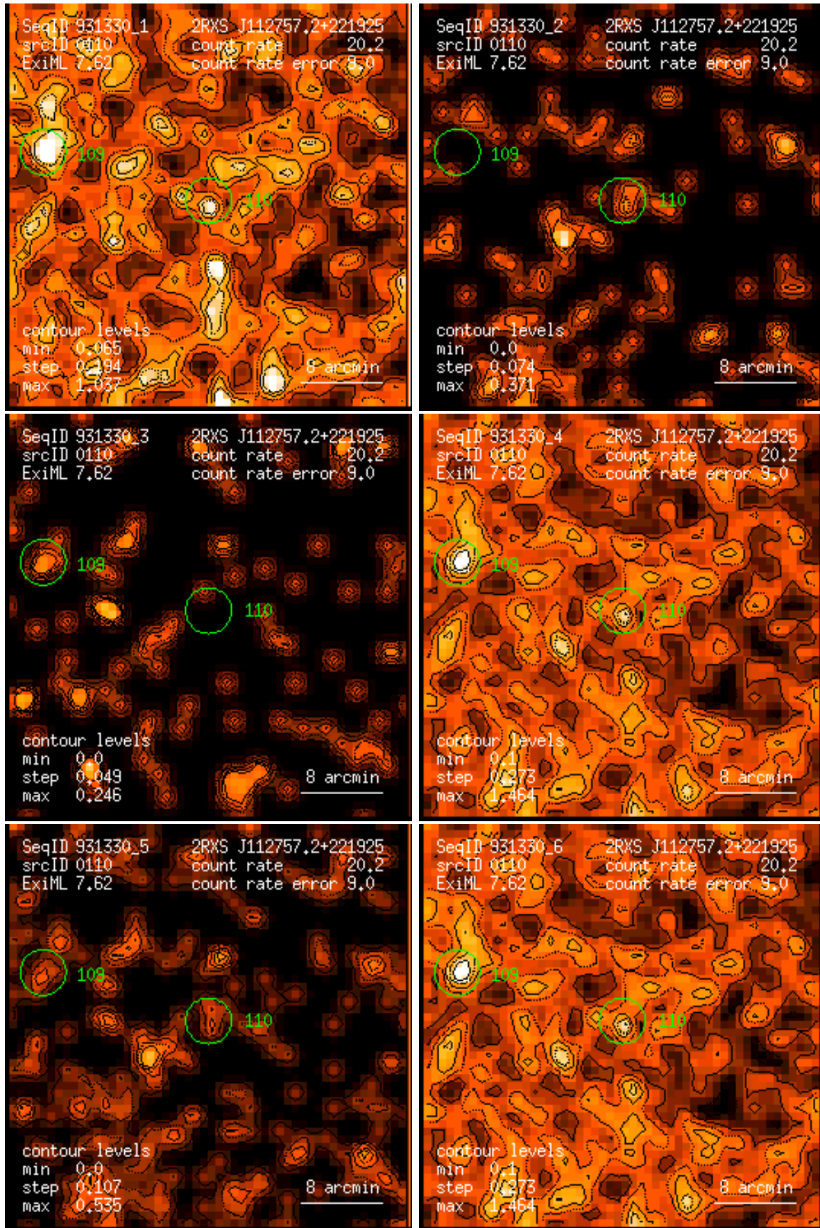
Figure 110: RASS 931330: detection 0110: band rate images, Gaussian filter: (1) PSPC channels 11 – 41, (2) 52 – 90, (3) 91 – 201, (4) 11 – 235, (5) 52 – 201, (6) 11 – 201. Broad band rates in counts/ks. Band rate contour levels in counts/ks/arcmin 2 .
