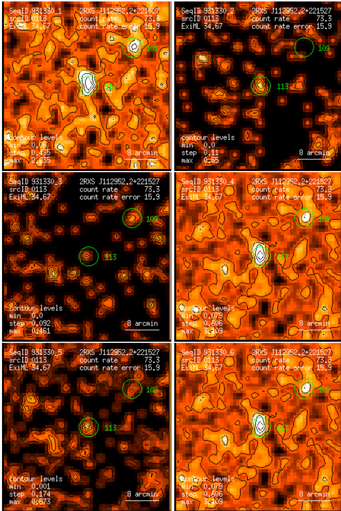
Figure 113: RASS 931330: detection 0113: band rate images, Gaussian filter: (1) PSPC channels 11 – 41, (2) 52 – 90, (3) 91 – 201, (4) 11 – 235, (5) 52 – 201, (6) 11 – 201. Broad band rates in counts/ks. Band rate contour levels in counts/ks/arcmin 2 .
