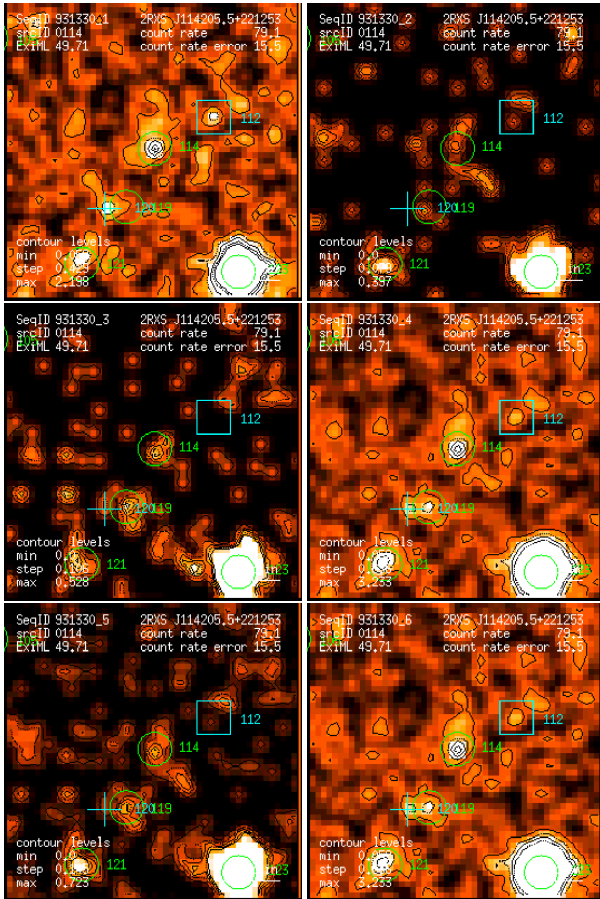
Figure 114: RASS 931330: detection 0114: band rate images, Gaussian filter: (1) PSPC channels 11 – 41, (2) 52 – 90, (3) 91 – 201, (4) 11 – 235, (5) 52 – 201, (6) 11 – 201. Broad band rates in counts/ks. Band rate contour levels in counts/ks/arcmin 2 .
