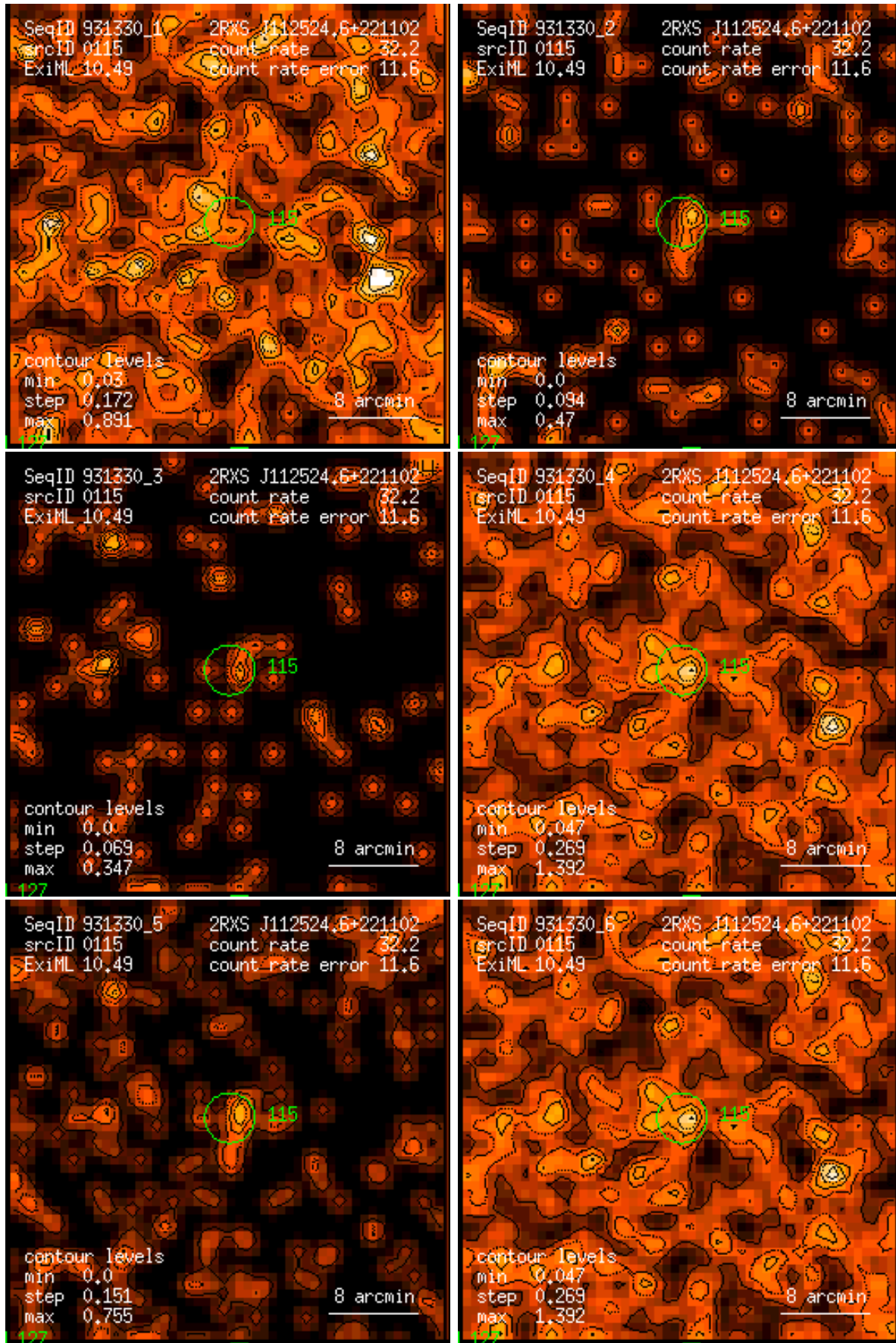
Figure 115: RASS 931330: detection 0115: band rate images, Gaussian filter: (1) PSPC channels 11 – 41, (2) 52 – 90, (3) 91 – 201, (4) 11 – 235, (5) 52 – 201, (6) 11 – 201. Broad band rates in counts/ks. Band rate contour levels in counts/ks/arcmin 2 .
