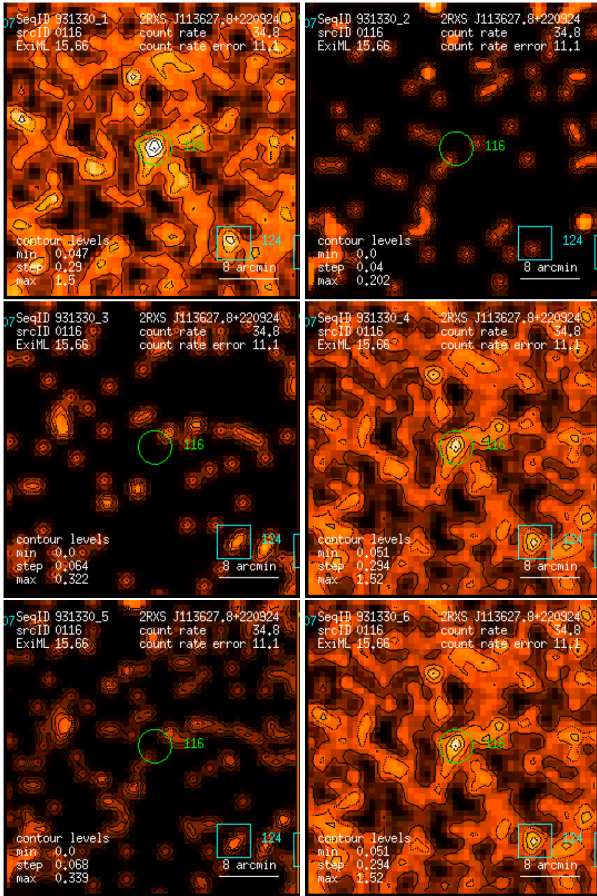
Figure 116: RASS 931330: detection 0116: band rate images, Gaussian filter: (1) PSPC channels 11 – 41, (2) 52 – 90, (3) 91 – 201, (4) 11 – 235, (5) 52 – 201, (6) 11 – 201. Broad band rates in counts/ks. Band rate contour levels in counts/ks/arcmin 2 .
