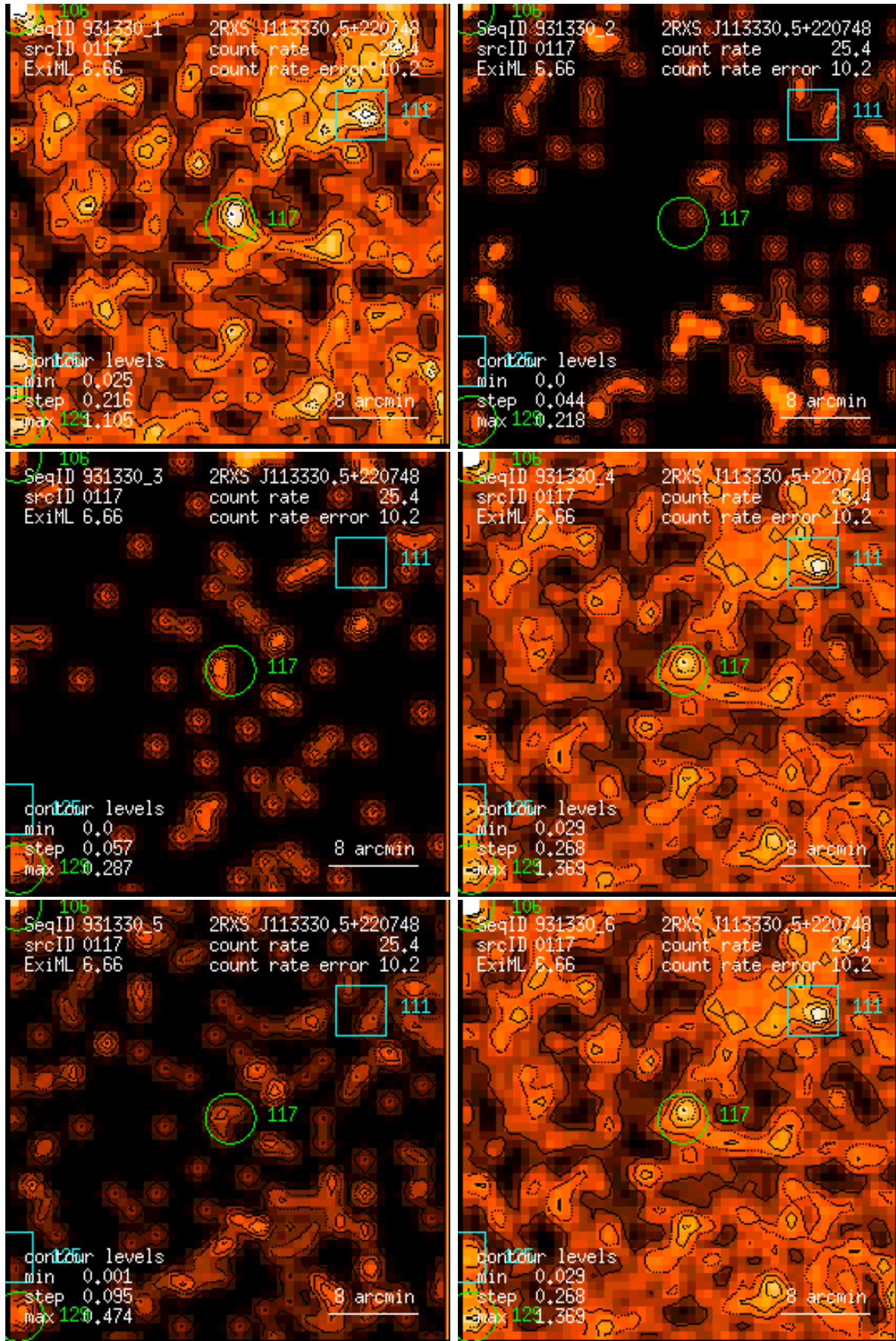
Figure 117: RASS 931330: detection 0117: band rate images, Gaussian filter: (1) PSPC channels 11 – 41, (2) 52 – 90, (3) 91 – 201, (4) 11 – 235, (5) 52 – 201, (6) 11 – 201. Broad band rates in counts/ks. Band rate contour levels in counts/ks/arcmin 2 .
