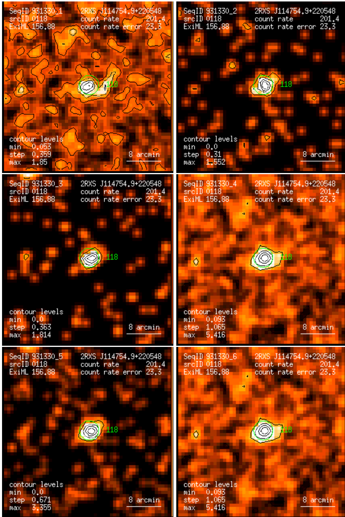
Figure 118: RASS 931330: detection 0118: band rate images, Gaussian filter: (1) PSPC channels 11 – 41, (2) 52 – 90, (3) 91 – 201, (4) 11 – 235, (5) 52 – 201, (6) 11 – 201. Broad band rates in counts/ks. Band rate contour levels in counts/ks/arcmin 2 .
