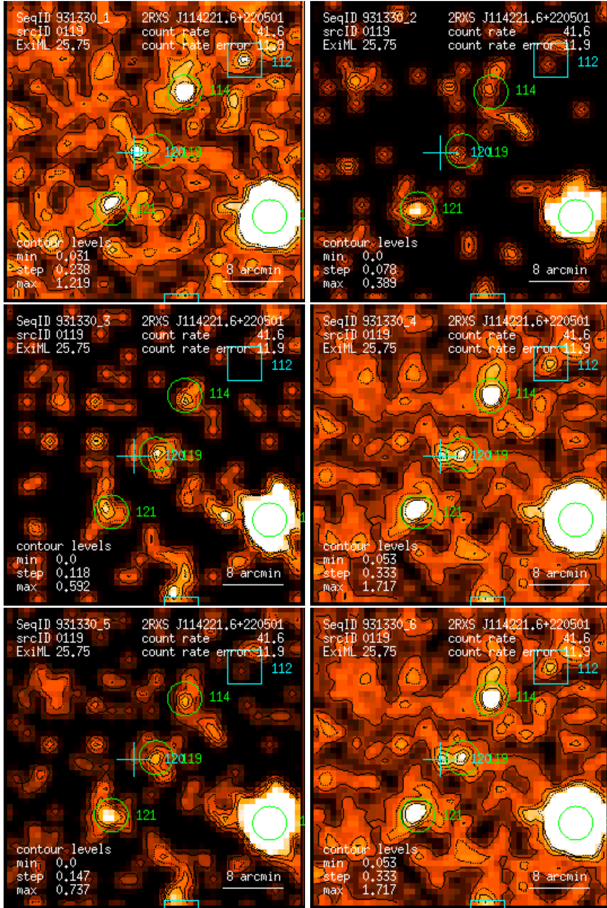
Figure 119: RASS 931330: detection 0119: band rate images, Gaussian filter: (1) PSPC channels 11 – 41, (2) 52 – 90, (3) 91 – 201, (4) 11 – 235, (5) 52 – 201, (6) 11 – 201. Broad band rates in counts/ks. Band rate contour levels in counts/ks/arcmin 2 .
