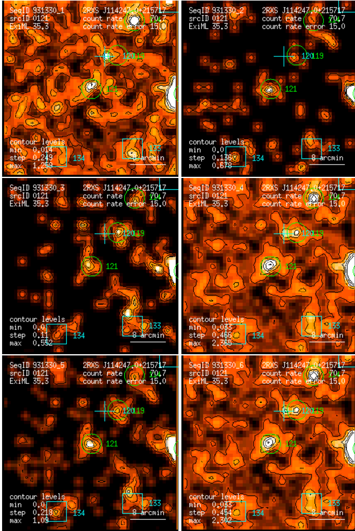
Figure 121: RASS 931330: detection 0121: band rate images, Gaussian filter: (1) PSPC channels 11 – 41, (2) 52 – 90, (3) 91 – 201, (4) 11 – 235, (5) 52 – 201, (6) 11 – 201. Broad band rates in counts/ks. Band rate contour levels in counts/ks/arcmin 2 .
