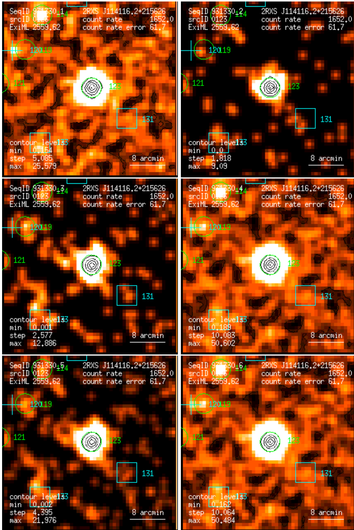
Figure 123: RASS 931330: detection 0123: band rate images, Gaussian filter: (1) PSPC channels 11 – 41, (2) 52 – 90, (3) 91 – 201, (4) 11 – 235, (5) 52 – 201, (6) 11 – 201. Broad band rates in counts/ks. Band rate contour levels in counts/ks/arcmin 2 .
