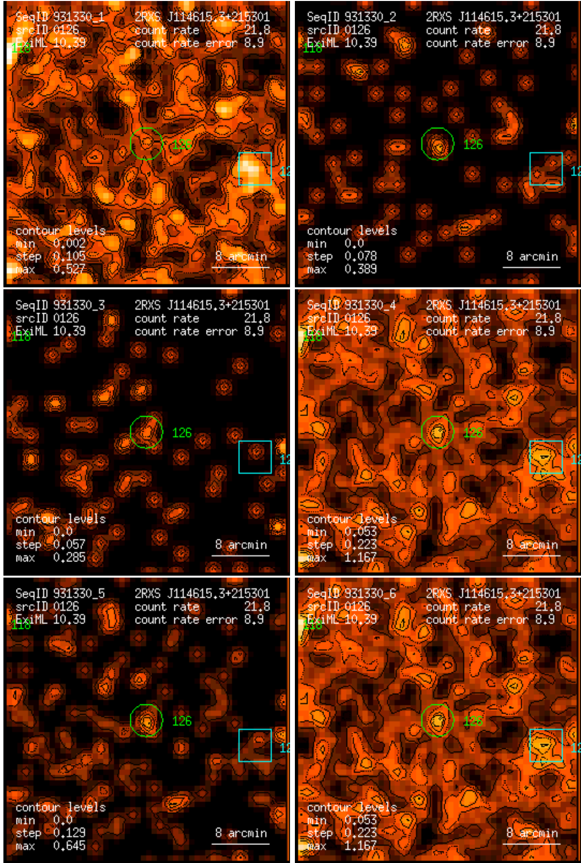
Figure 126: RASS 931330: detection 0126: band rate images, Gaussian filter: (1) PSPC channels 11 – 41, (2) 52 – 90, (3) 91 – 201, (4) 11 – 235, (5) 52 – 201, (6) 11 – 201. Broad band rates in counts/ks. Band rate contour levels in counts/ks/arcmin 2 .
