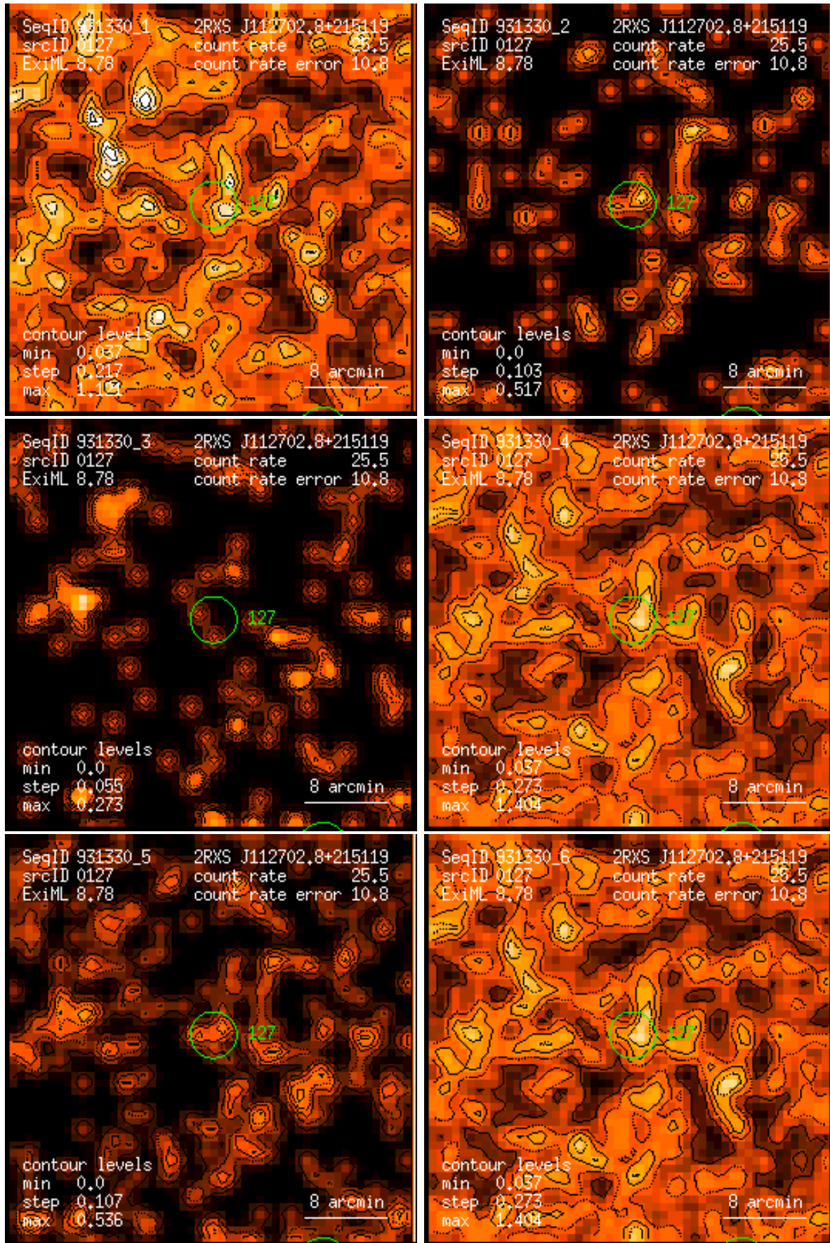
Figure 127: RASS 931330: detection 0127: band rate images, Gaussian filter: (1) PSPC channels 11 – 41, (2) 52 – 90, (3) 91 – 201, (4) 11 – 235, (5) 52 – 201, (6) 11 – 201. Broad band rates in counts/ks. Band rate contour levels in counts/ks/arcmin 2 .
