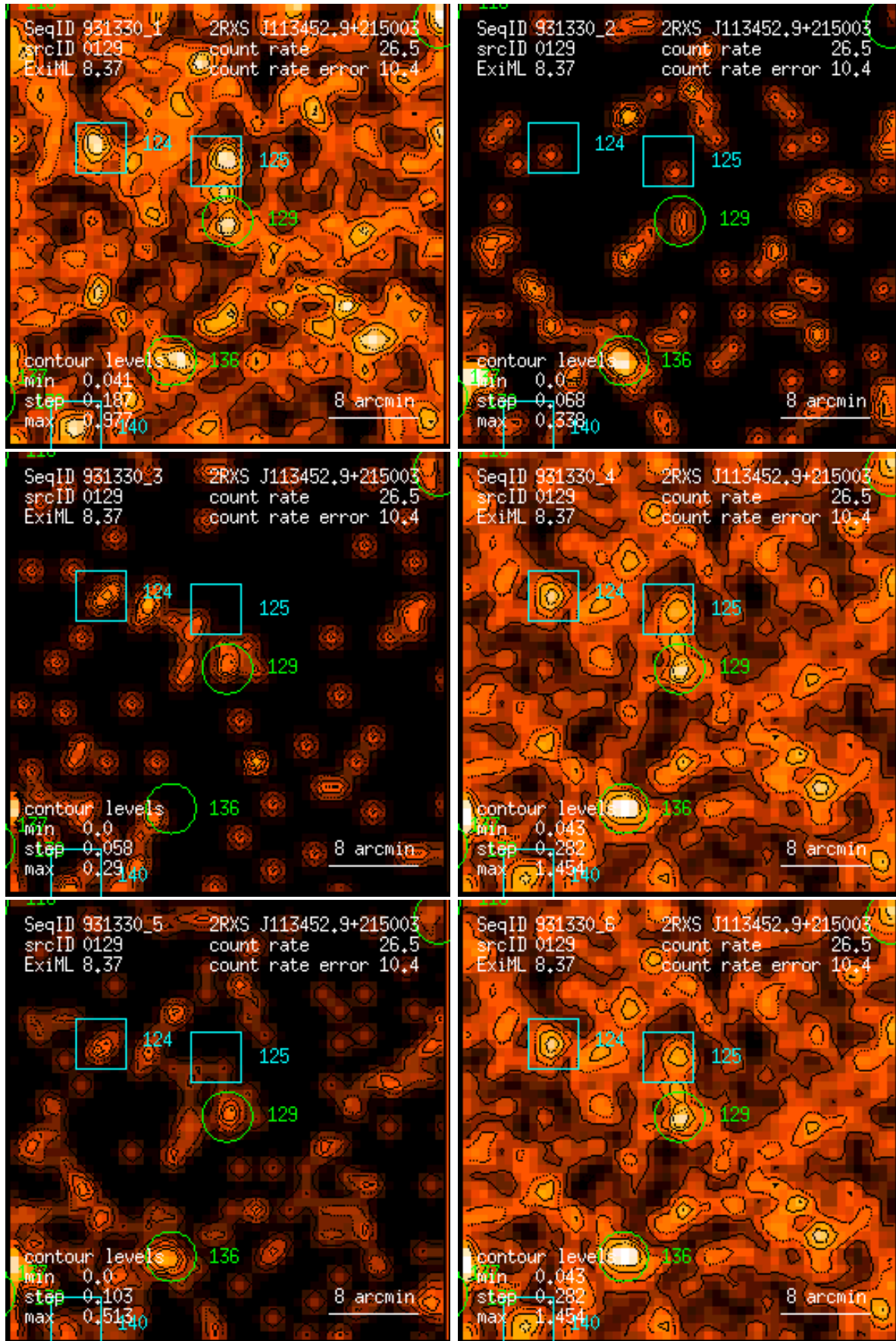
Figure 129: RASS 931330: detection 0129: band rate images, Gaussian filter: (1) PSPC channels 11 – 41, (2) 52 – 90, (3) 91 – 201, (4) 11 – 235, (5) 52 – 201, (6) 11 – 201. Broad band rates in counts/ks. Band rate contour levels in counts/ks/arcmin 2 .
