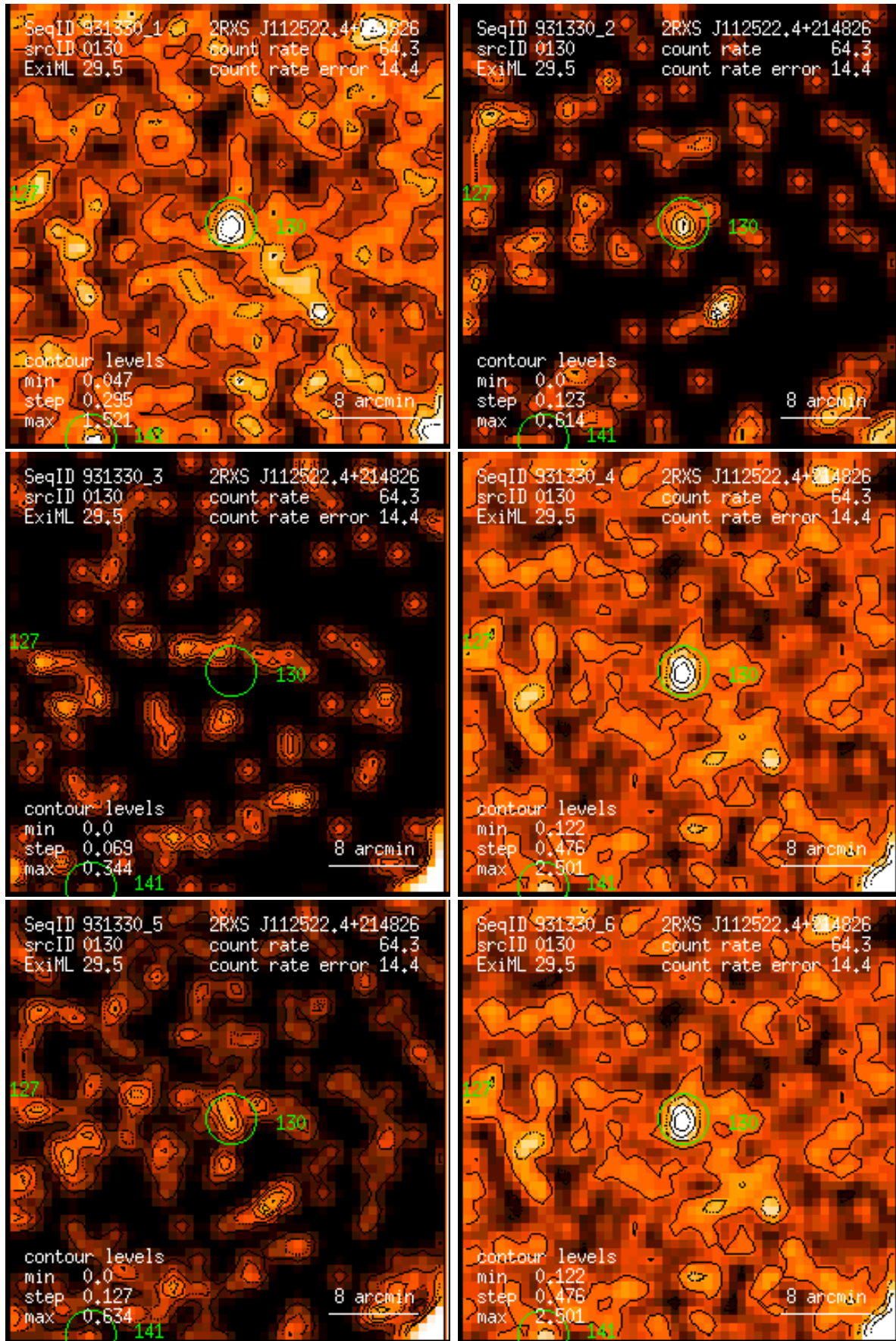
Figure 130: RASS 931330: detection 0130: band rate images, Gaussian filter: (1) PSPC channels 11 – 41, (2) 52 – 90, (3) 91 – 201, (4) 11 – 235, (5) 52 – 201, (6) 11 – 201. Broad band rates in counts/ks. Band rate contour levels in counts/ks/arcmin 2 .
