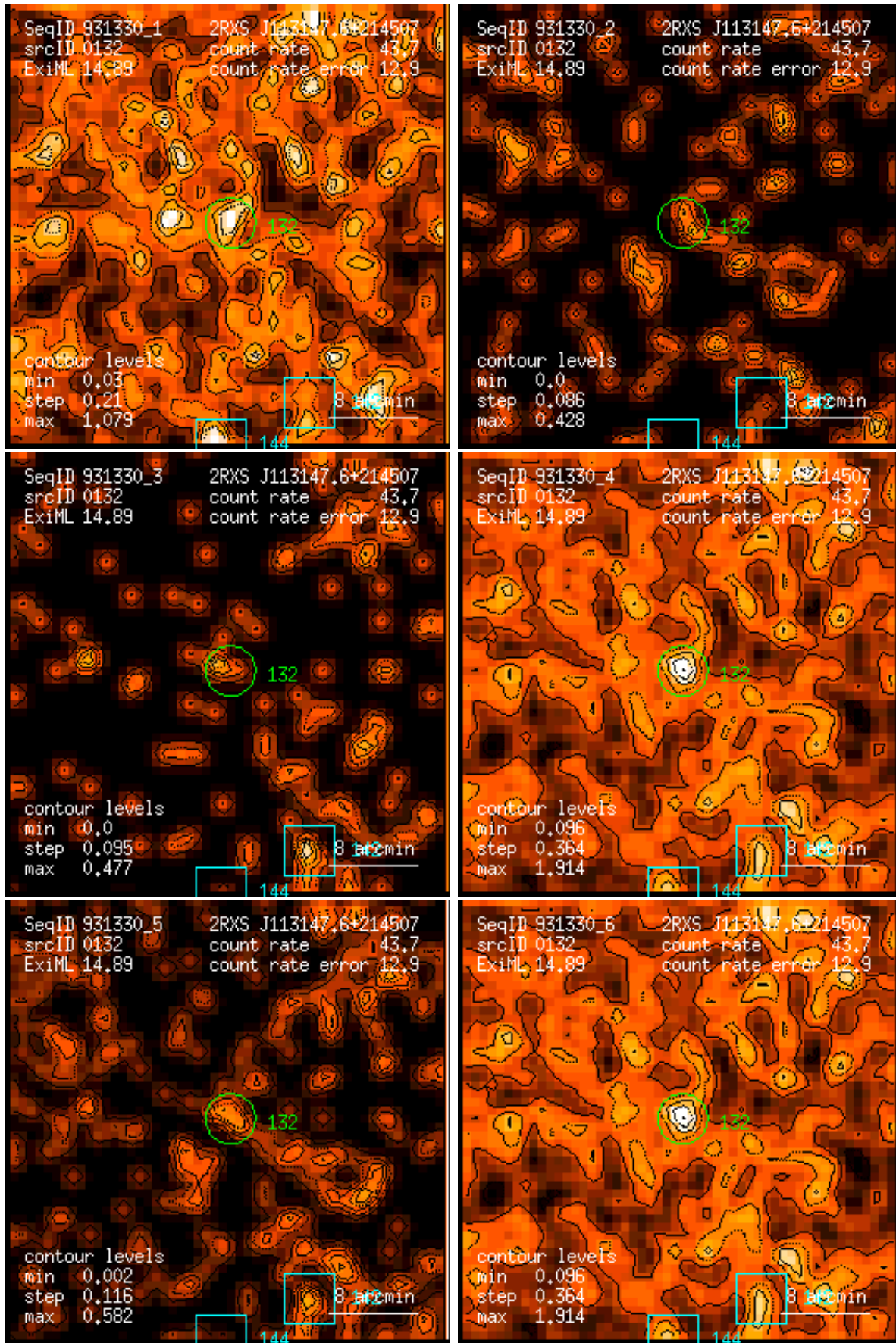
Figure 132: RASS 931330: detection 0132: band rate images, Gaussian filter: (1) PSPC channels 11 – 41, (2) 52 – 90, (3) 91 – 201, (4) 11 – 235, (5) 52 – 201, (6) 11 – 201. Broad band rates in counts/ks. Band rate contour levels in counts/ks/arcmin 2 .
