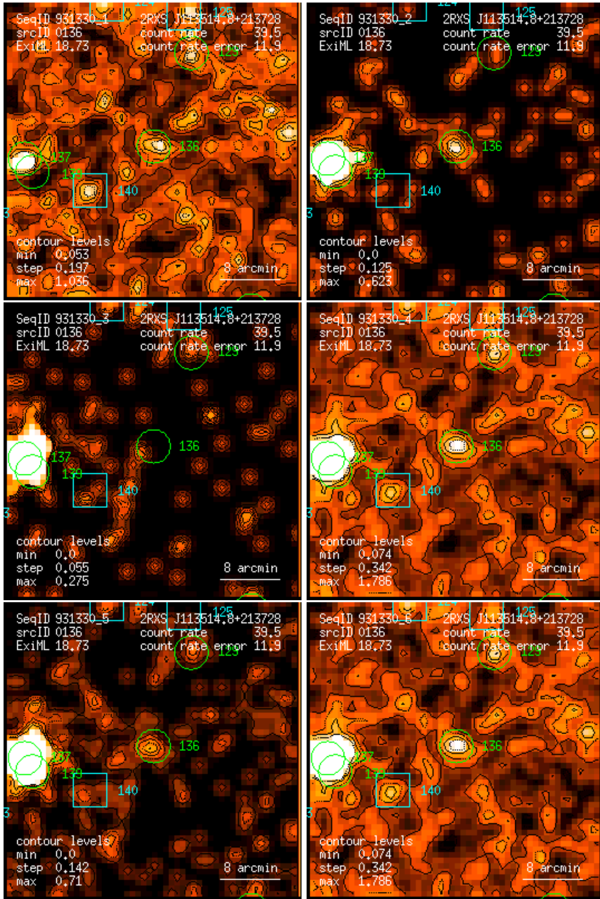
Figure 136: RASS 931330: detection 0136: band rate images, Gaussian filter: (1) PSPC channels 11 – 41, (2) 52 – 90, (3) 91 – 201, (4) 11 – 235, (5) 52 – 201, (6) 11 – 201. Broad band rates in counts/ks. Band rate contour levels in counts/ks/arcmin 2 .
