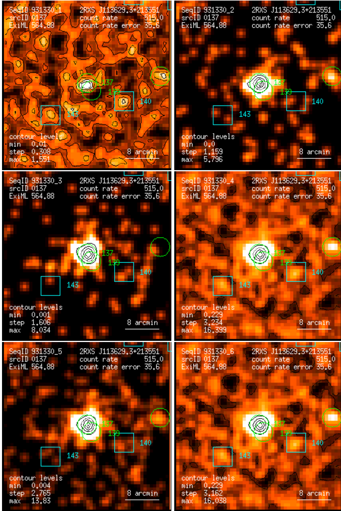
Figure 137: RASS 931330: detection 0137: band rate images, Gaussian filter: (1) PSPC channels 11 – 41, (2) 52 – 90, (3) 91 – 201, (4) 11 – 235, (5) 52 – 201, (6) 11 – 201. Broad band rates in counts/ks. Band rate contour levels in counts/ks/arcmin 2 .
