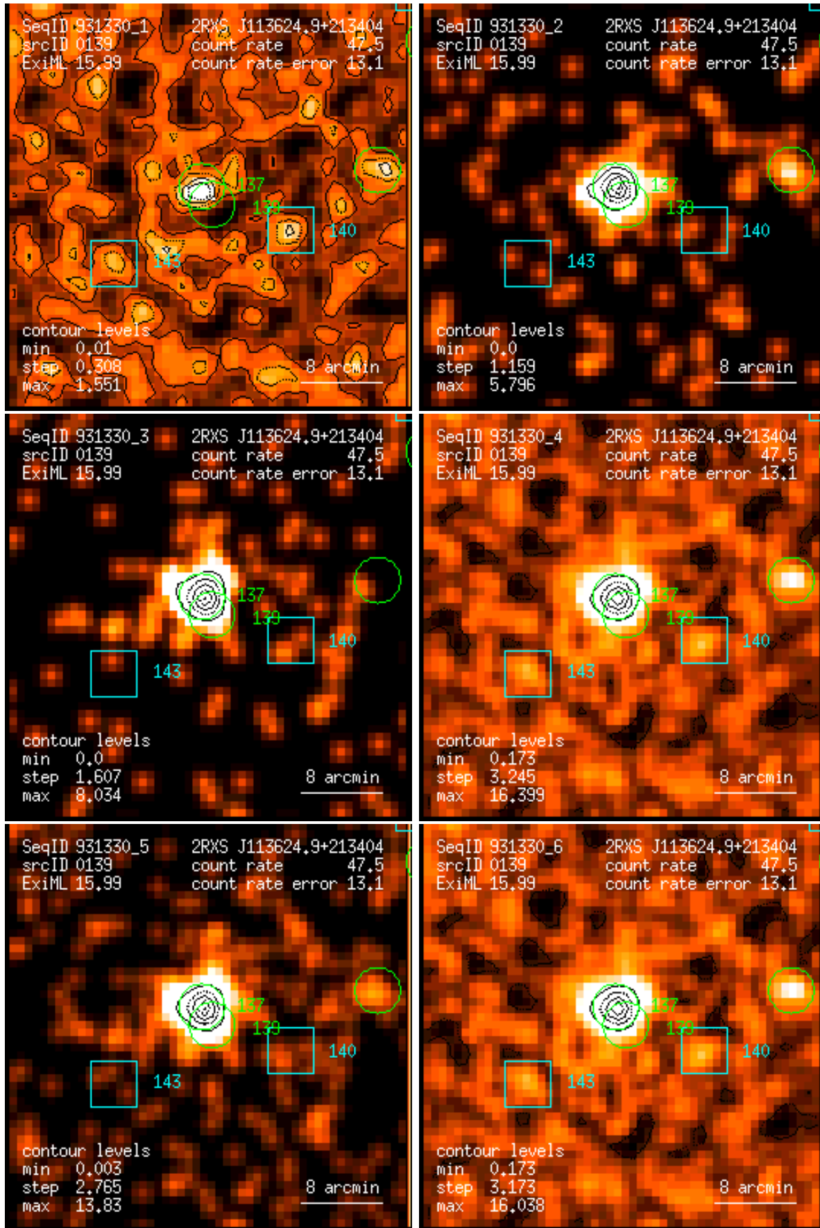
Figure 139: RASS 931330: detection 0139: band rate images, Gaussian filter: (1) PSPC channels 11 – 41, (2) 52 – 90, (3) 91 – 201, (4) 11 – 235, (5) 52 – 201, (6) 11 – 201. Broad band rates in counts/ks. Band rate contour levels in counts/ks/arcmin 2 .
