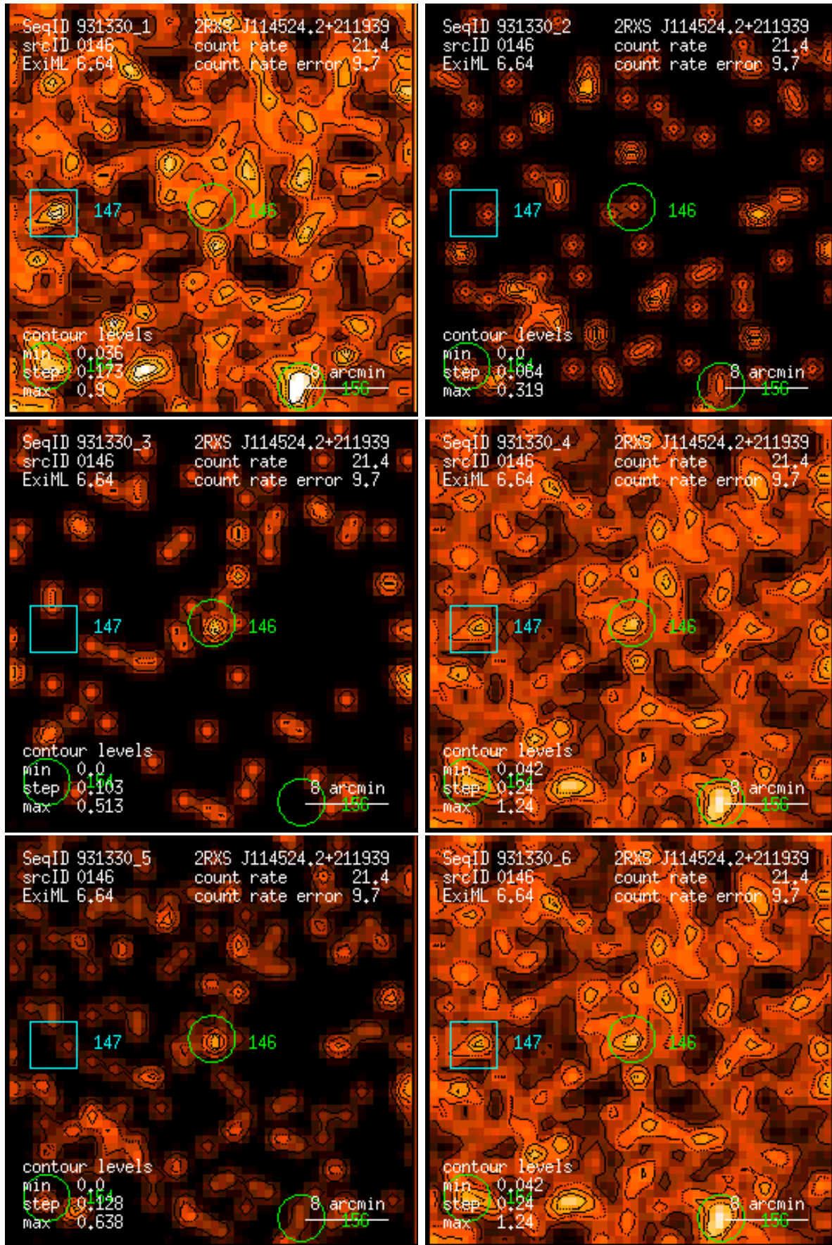
Figure 146: RASS 931330: detection 0146: band rate images, Gaussian filter: (1) PSPC channels 11 – 41, (2) 52 – 90, (3) 91 – 201, (4) 11 – 235, (5) 52 – 201, (6) 11 – 201. Broad band rates in counts/ks. Band rate contour levels in counts/ks/arcmin 2 .
