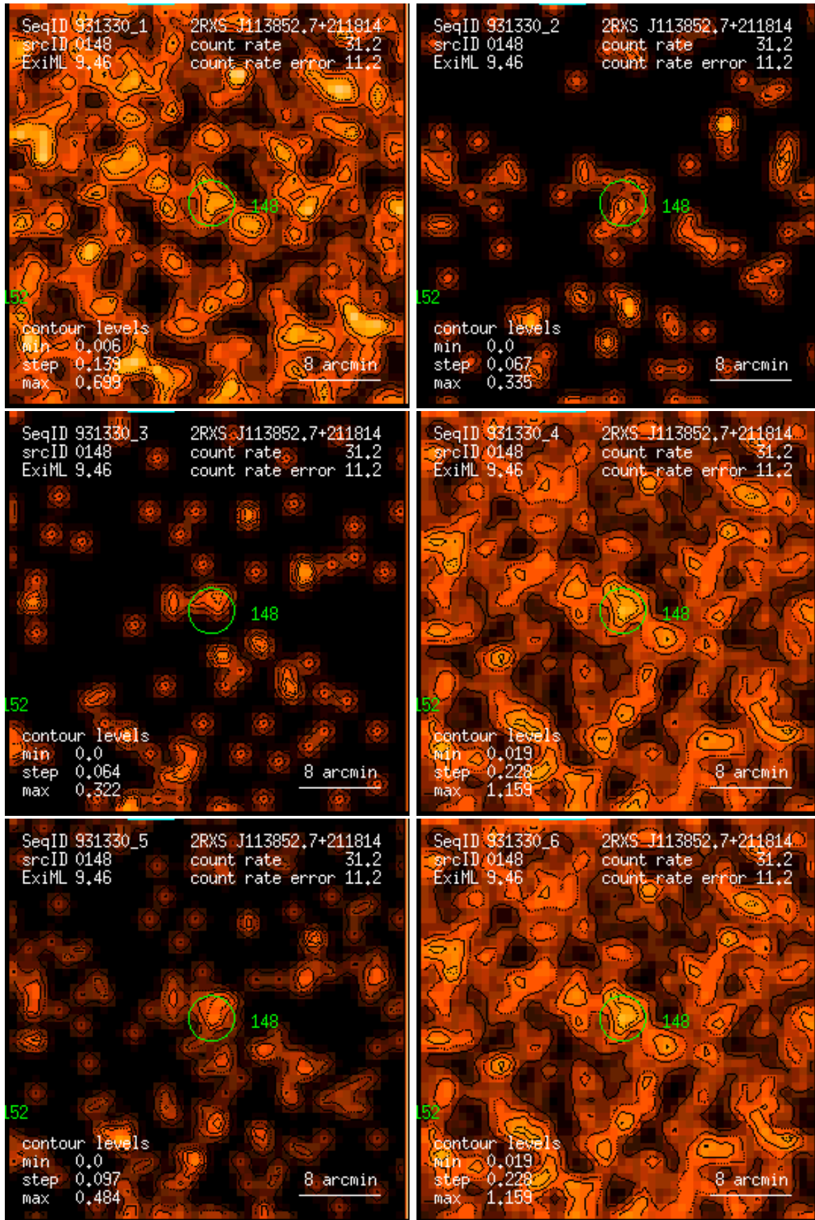
Figure 148: RASS 931330: detection 0148: band rate images, Gaussian filter: (1) PSPC channels 11 – 41, (2) 52 – 90, (3) 91 – 201, (4) 11 – 235, (5) 52 – 201, (6) 11 – 201. Broad band rates in counts/ks. Band rate contour levels in counts/ks/arcmin 2 .
