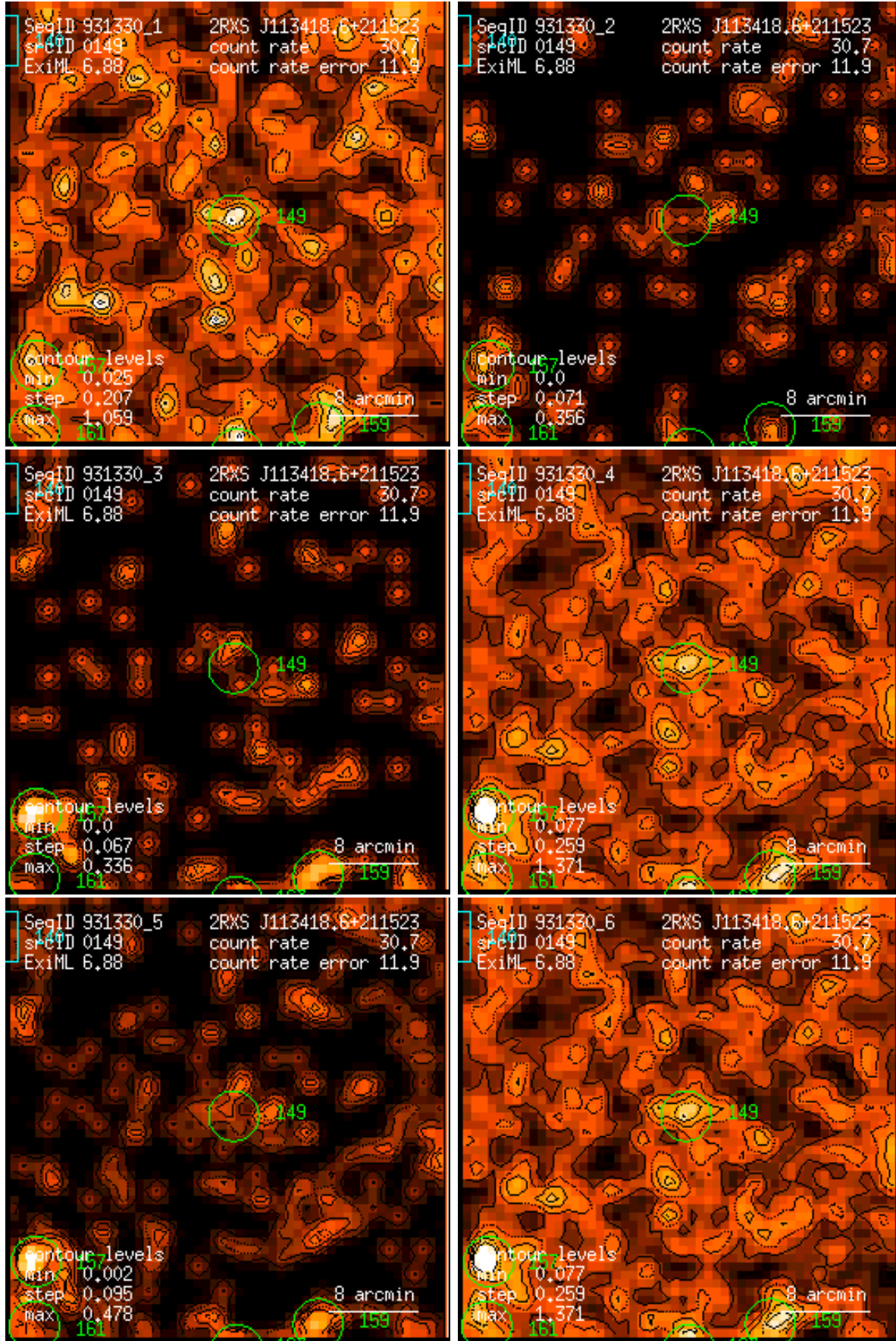
Figure 149: RASS 931330: detection 0149: band rate images, Gaussian filter: (1) PSPC channels 11 – 41, (2) 52 – 90, (3) 91 – 201, (4) 11 – 235, (5) 52 – 201, (6) 11 – 201. Broad band rates in counts/ks. Band rate contour levels in counts/ks/arcmin 2 .
