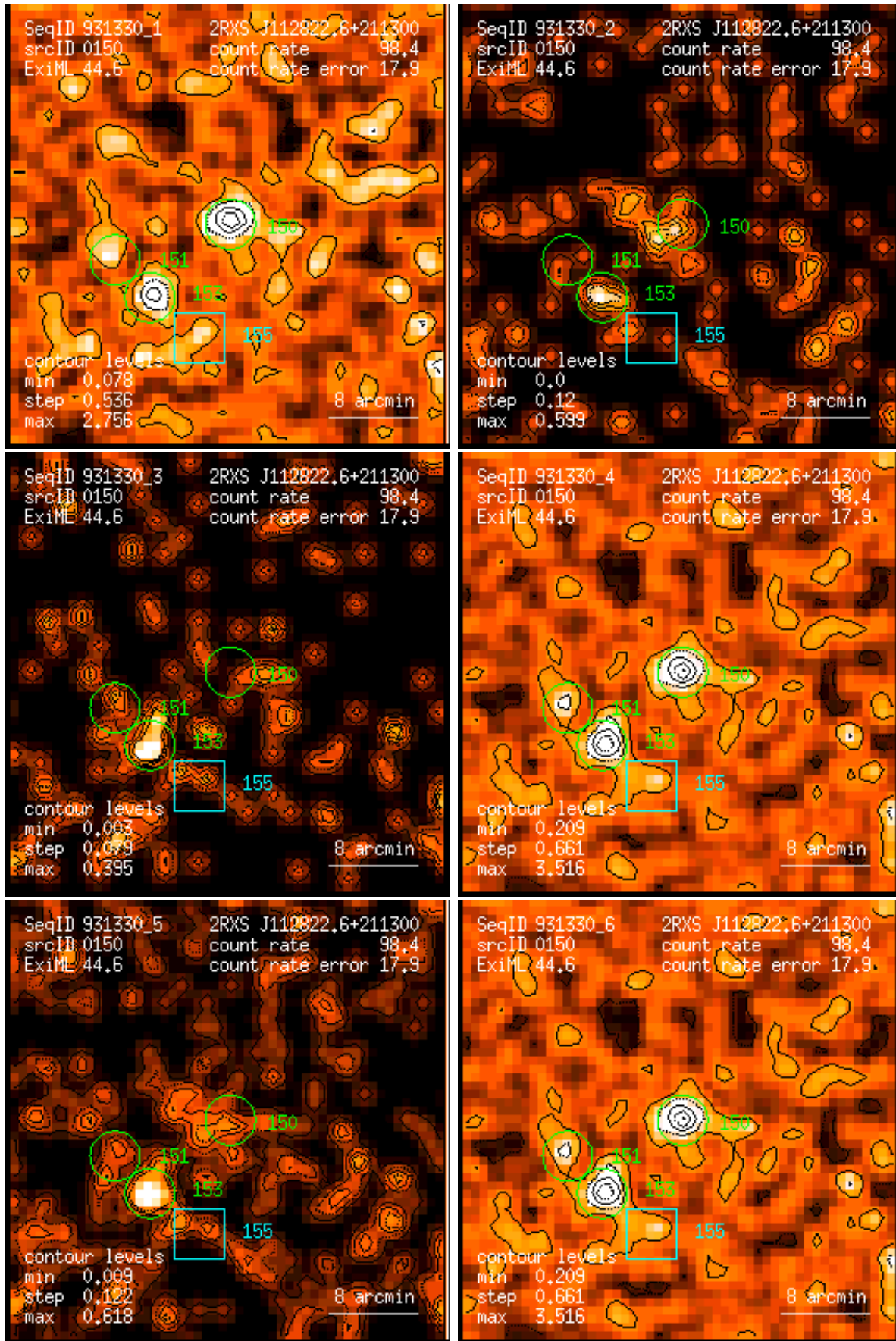
Figure 150: RASS 931330: detection 0150: band rate images, Gaussian filter: (1) PSPC channels 11 – 41, (2) 52 – 90, (3) 91 – 201, (4) 11 – 235, (5) 52 – 201, (6) 11 – 201. Broad band rates in counts/ks. Band rate contour levels in counts/ks/arcmin 2 .
