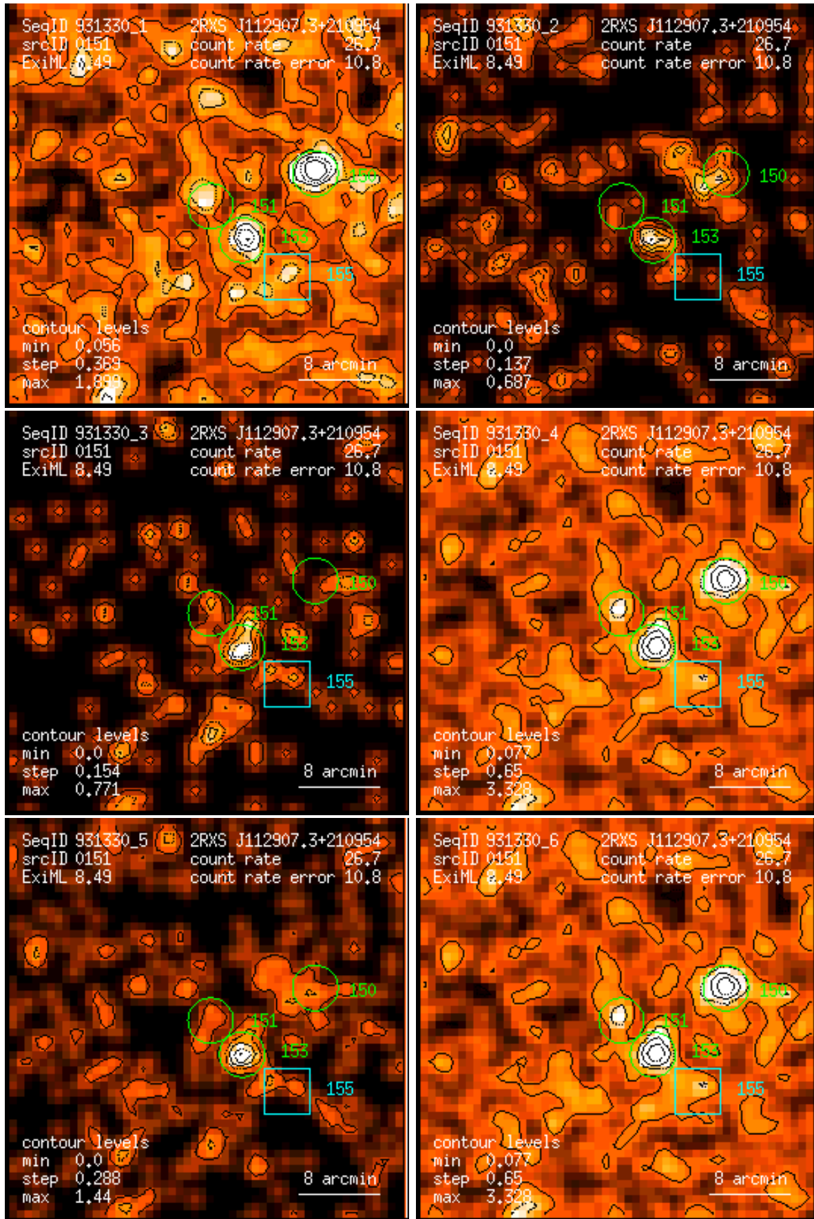
Figure 151: RASS 931330: detection 0151: band rate images, Gaussian filter: (1) PSPC channels 11 – 41, (2) 52 – 90, (3) 91 – 201, (4) 11 – 235, (5) 52 – 201, (6) 11 – 201. Broad band rates in counts/ks. Band rate contour levels in counts/ks/arcmin 2 .
