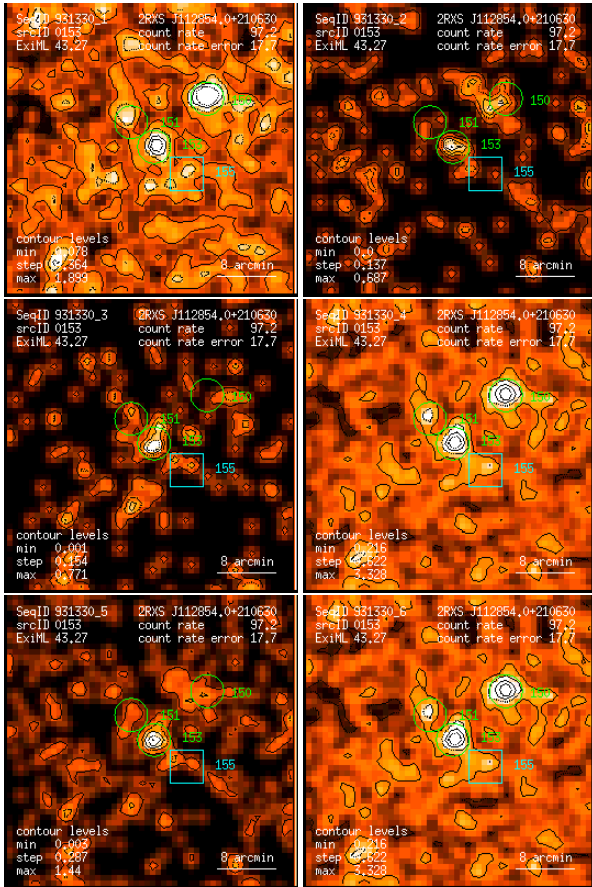
Figure 153: RASS 931330: detection 0153: band rate images, Gaussian filter: (1) PSPC channels 11 – 41, (2) 52 – 90, (3) 91 – 201, (4) 11 – 235, (5) 52 – 201, (6) 11 – 201. Broad band rates in counts/ks. Band rate contour levels in counts/ks/arcmin 2 .
