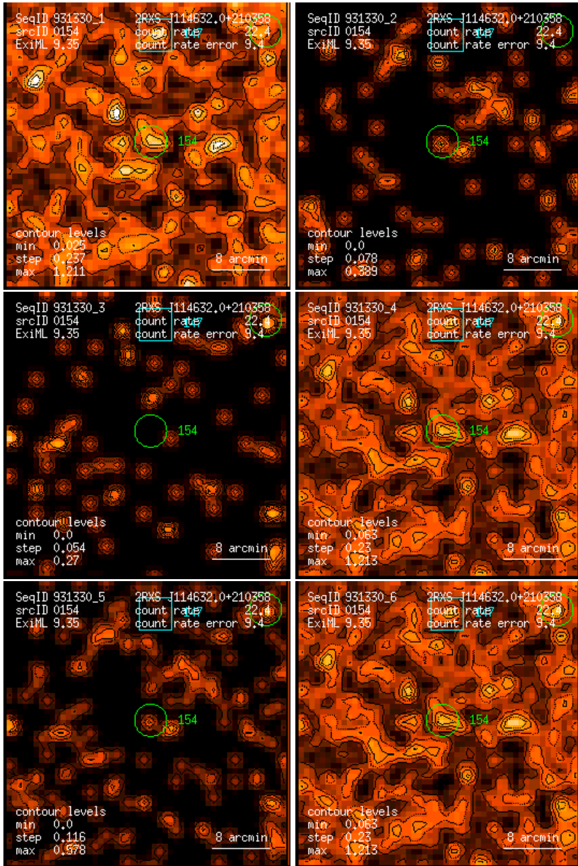
Figure 154: RASS 931330: detection 0154: band rate images, Gaussian filter: (1) PSPC channels 11 – 41, (2) 52 – 90, (3) 91 – 201, (4) 11 – 235, (5) 52 – 201, (6) 11 – 201. Broad band rates in counts/ks. Band rate contour levels in counts/ks/arcmin 2 .
