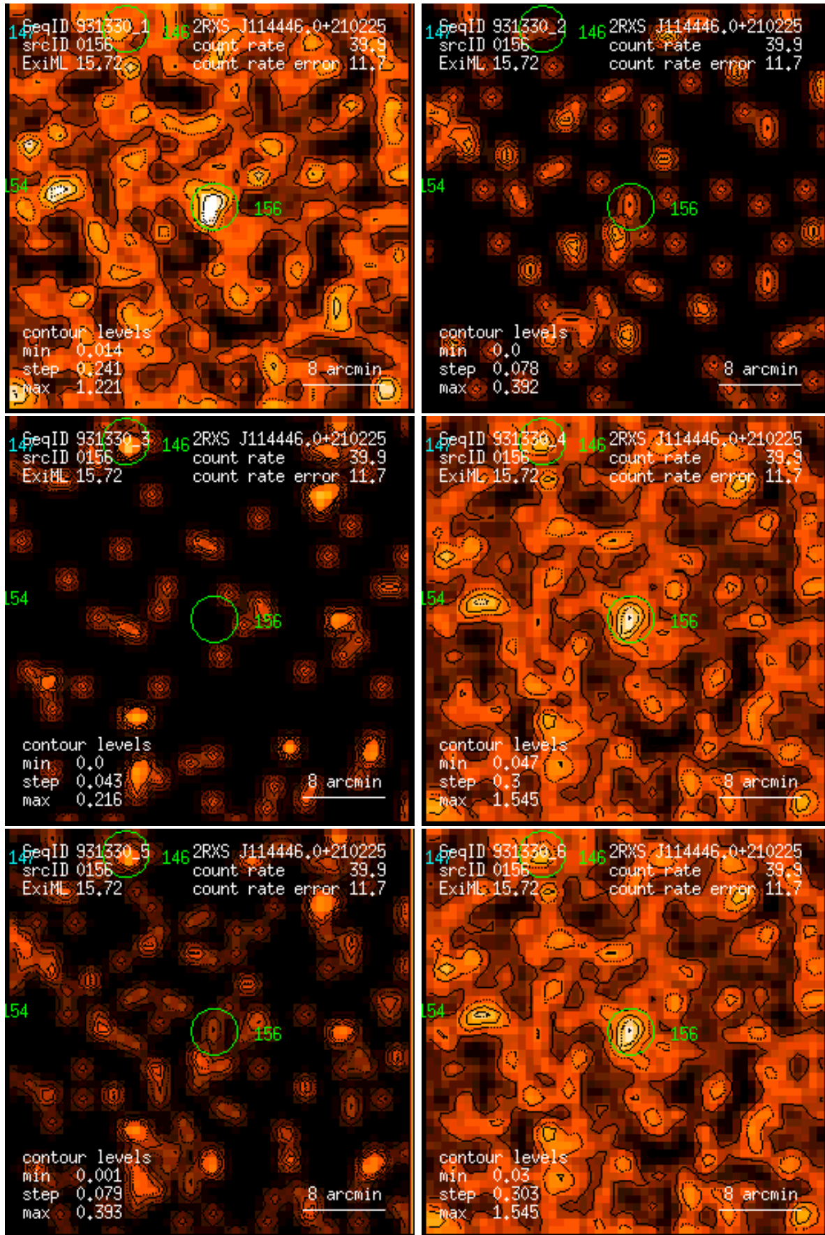
Figure 156: RASS 931330: detection 0156: band rate images, Gaussian filter: (1) PSPC channels 11 – 41, (2) 52 – 90, (3) 91 – 201, (4) 11 – 235, (5) 52 – 201, (6) 11 – 201. Broad band rates in counts/ks. Band rate contour levels in counts/ks/arcmin 2 .
