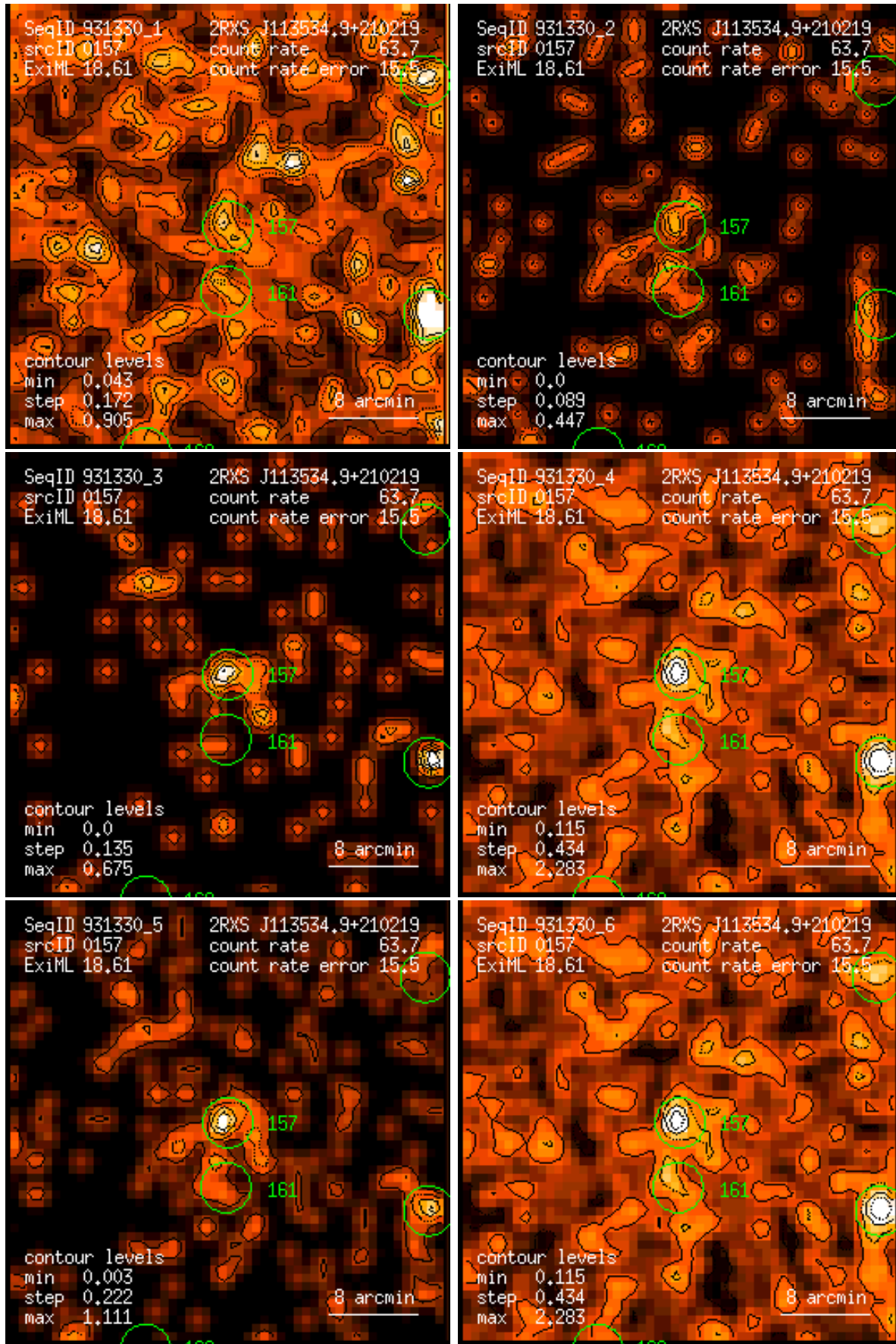
Figure 157: RASS 931330: detection 0157: band rate images, Gaussian filter: (1) PSPC channels 11 – 41, (2) 52 – 90, (3) 91 – 201, (4) 11 – 235, (5) 52 – 201, (6) 11 – 201. Broad band rates in counts/ks. Band rate contour levels in counts/ks/arcmin 2 .
