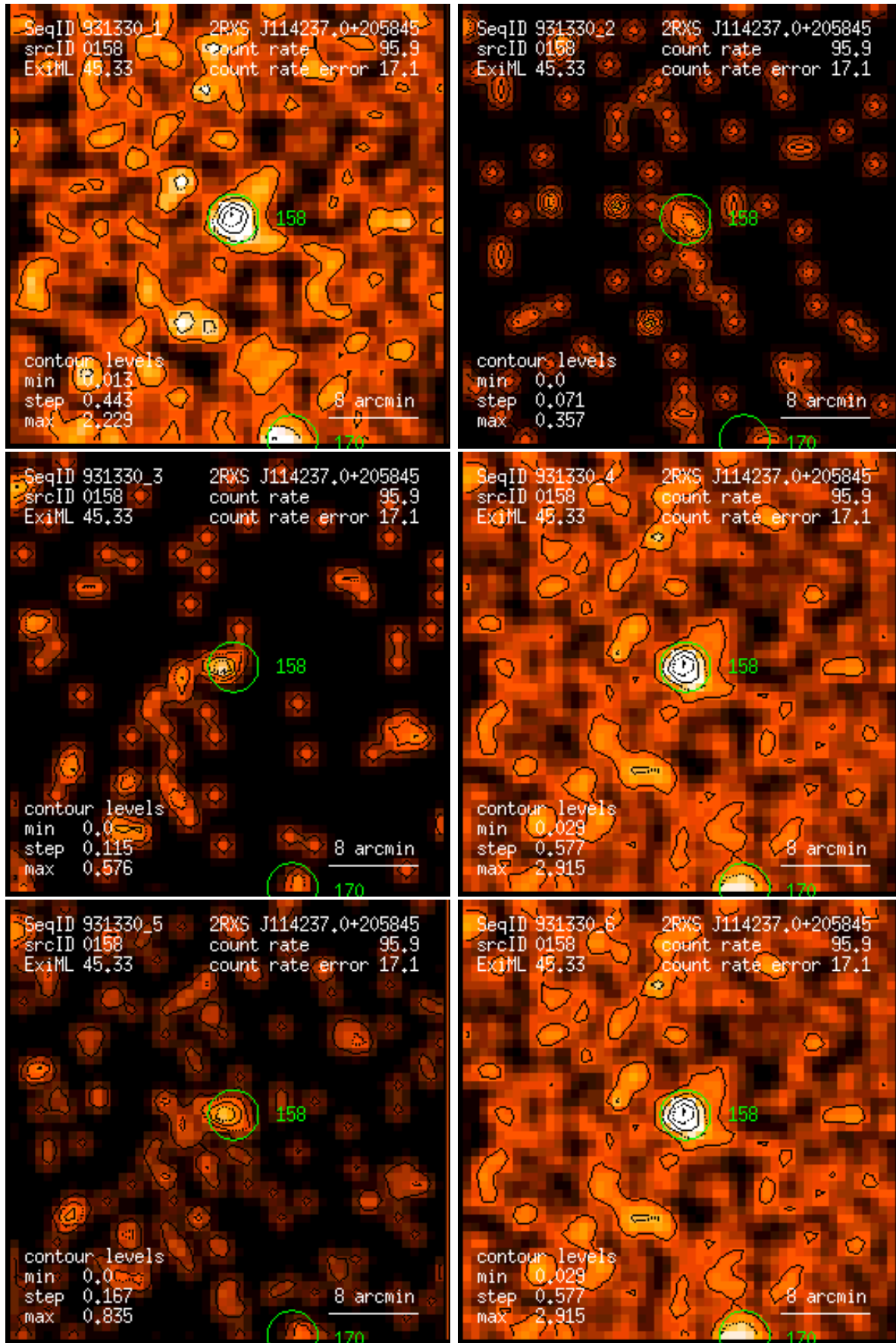
Figure 158: RASS 931330: detection 0158: band rate images, Gaussian filter: (1) PSPC channels 11 – 41, (2) 52 – 90, (3) 91 – 201, (4) 11 – 235, (5) 52 – 201, (6) 11 – 201. Broad band rates in counts/ks. Band rate contour levels in counts/ks/arcmin 2 .
