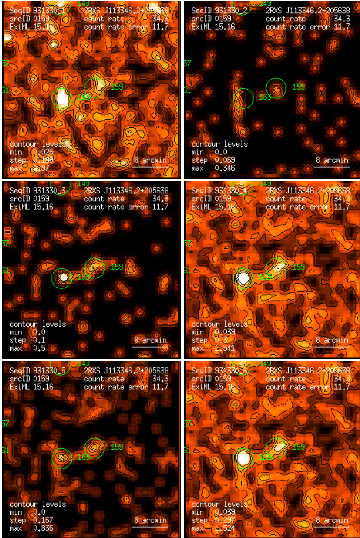
Figure 159: RASS 931330: detection 0159: band rate images, Gaussian filter: (1) PSPC channels 11 – 41, (2) 52 – 90, (3) 91 – 201, (4) 11 – 235, (5) 52 – 201, (6) 11 – 201. Broad band rates in counts/ks. Band rate contour levels in counts/ks/arcmin 2 .
