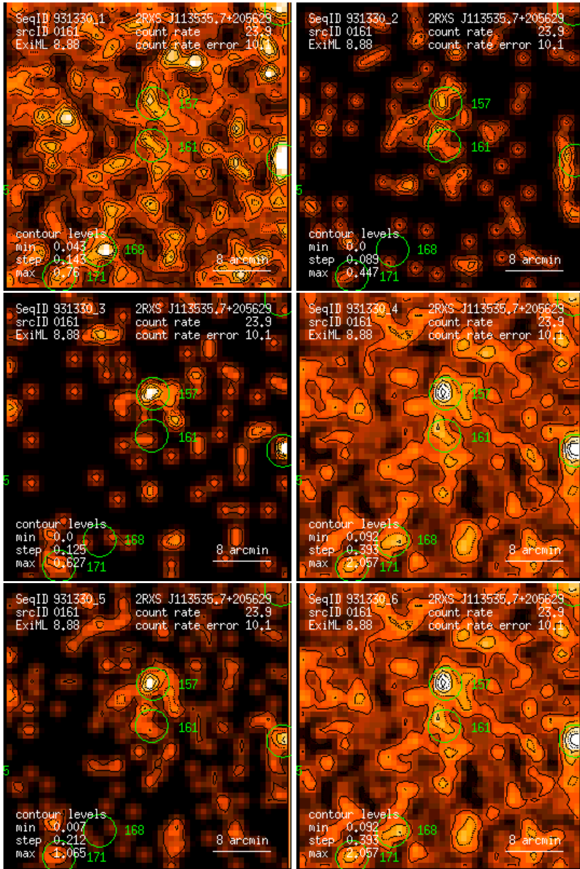
Figure 161: RASS 931330: detection 0161: band rate images, Gaussian filter: (1) PSPC channels 11 – 41, (2) 52 – 90, (3) 91 – 201, (4) 11 – 235, (5) 52 – 201, (6) 11 – 201. Broad band rates in counts/ks. Band rate contour levels in counts/ks/arcmin 2 .
