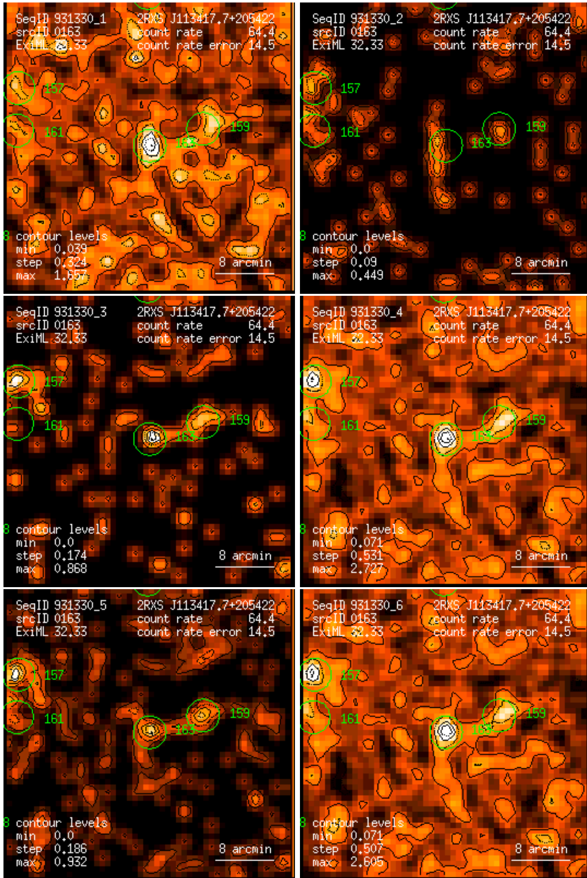
Figure 163: RASS 931330: detection 0163: band rate images, Gaussian filter: (1) PSPC channels 11 – 41, (2) 52 – 90, (3) 91 – 201, (4) 11 – 235, (5) 52 – 201, (6) 11 – 201. Broad band rates in counts/ks. Band rate contour levels in counts/ks/arcmin 2 .
