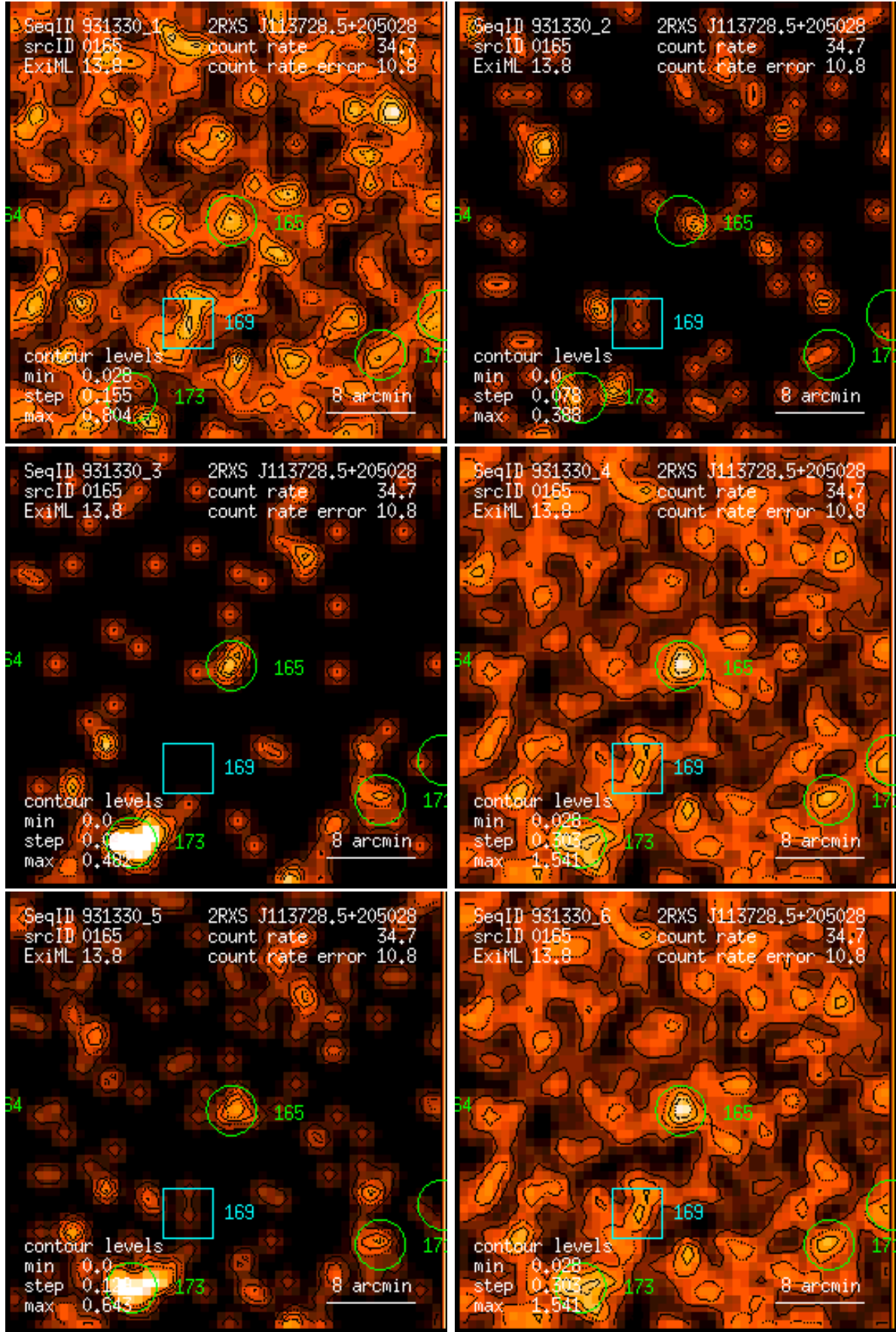
Figure 165: RASS 931330: detection 0165: band rate images, Gaussian filter: (1) PSPC channels 11 – 41, (2) 52 – 90, (3) 91 – 201, (4) 11 – 235, (5) 52 – 201, (6) 11 – 201. Broad band rates in counts/ks. Band rate contour levels in counts/ks/arcmin 2 .
