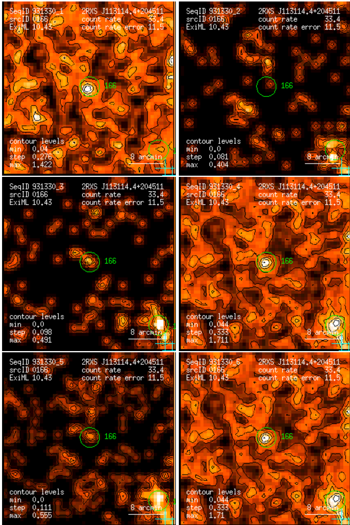
Figure 166: RASS 931330: detection 0166: band rate images, Gaussian filter: (1) PSPC channels 11 – 41, (2) 52 – 90, (3) 91 – 201, (4) 11 – 235, (5) 52 – 201, (6) 11 – 201. Broad band rates in counts/ks. Band rate contour levels in counts/ks/arcmin 2 .
