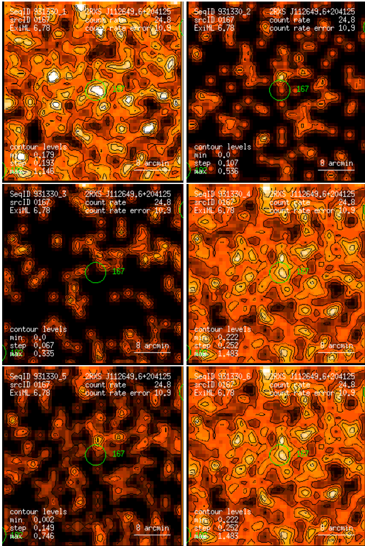
Figure 167: RASS 931330: detection 0167: band rate images, Gaussian filter: (1) PSPC channels 11 – 41, (2) 52 – 90, (3) 91 – 201, (4) 11 – 235, (5) 52 – 201, (6) 11 – 201. Broad band rates in counts/ks. Band rate contour levels in counts/ks/arcmin 2 .
