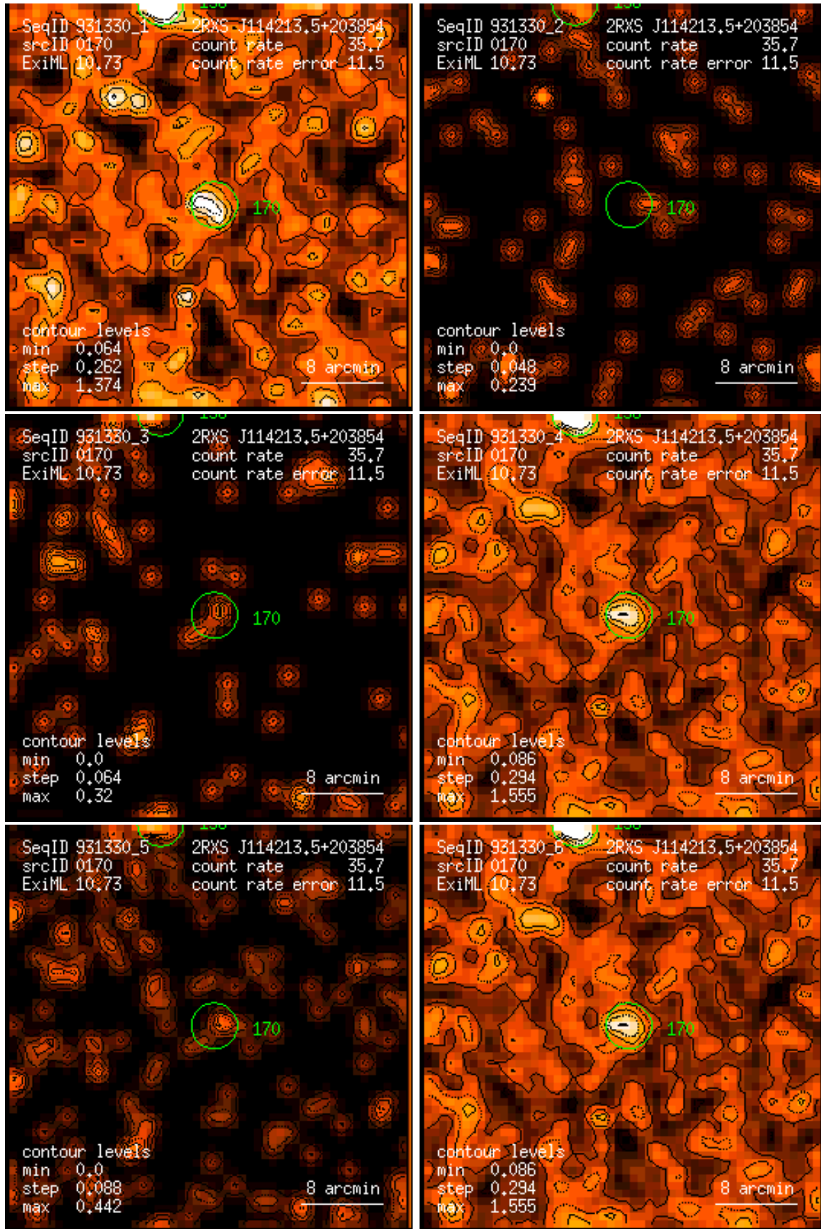
Figure 170: RASS 931330: detection 0170: band rate images, Gaussian filter: (1) PSPC channels 11 – 41, (2) 52 – 90, (3) 91 – 201, (4) 11 – 235, (5) 52 – 201, (6) 11 – 201. Broad band rates in counts/ks. Band rate contour levels in counts/ks/arcmin 2 .
