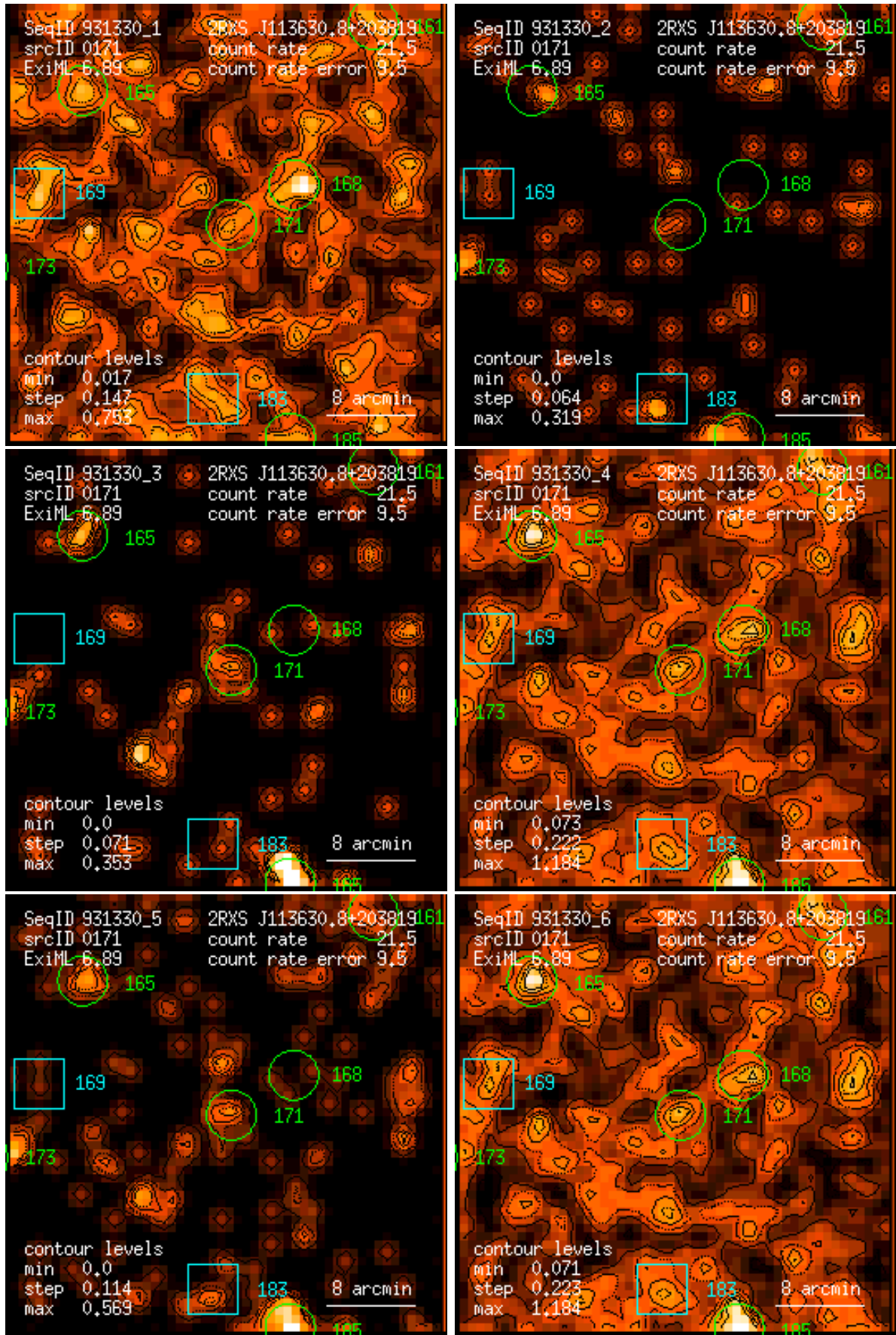
Figure 171: RASS 931330: detection 0171: band rate images, Gaussian filter: (1) PSPC channels 11 – 41, (2) 52 – 90, (3) 91 – 201, (4) 11 – 235, (5) 52 – 201, (6) 11 – 201. Broad band rates in counts/ks. Band rate contour levels in counts/ks/arcmin 2 .
