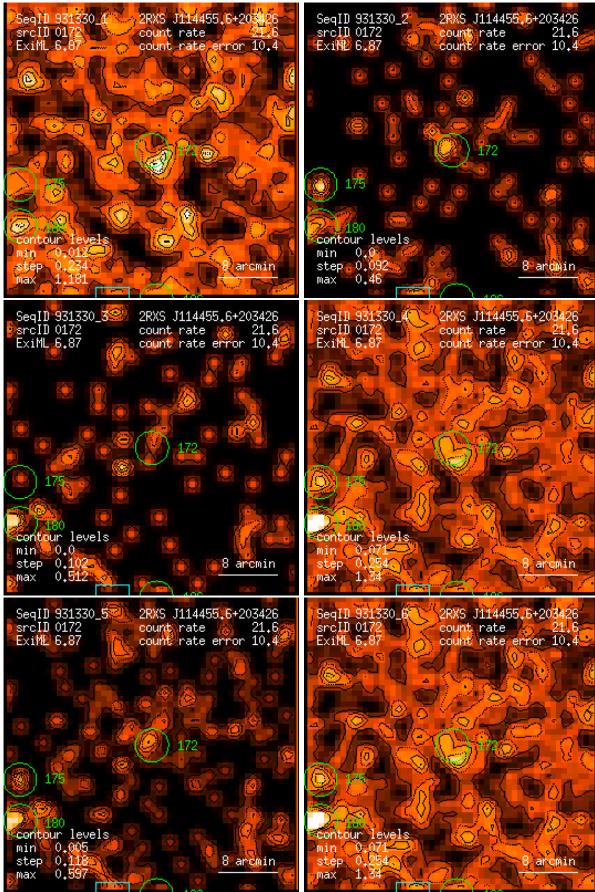
Figure 172: RASS 931330: detection 0172: band rate images, Gaussian filter: (1) PSPC channels 11 – 41, (2) 52 – 90, (3) 91 – 201, (4) 11 – 235, (5) 52 – 201, (6) 11 – 201. Broad band rates in counts/ks. Band rate contour levels in counts/ks/arcmin 2 .
