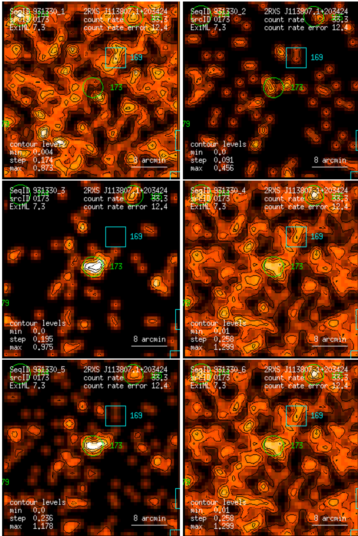
Figure 173: RASS 931330: detection 0173: band rate images, Gaussian filter: (1) PSPC channels 11 – 41, (2) 52 – 90, (3) 91 – 201, (4) 11 – 235, (5) 52 – 201, (6) 11 – 201. Broad band rates in counts/ks. Band rate contour levels in counts/ks/arcmin 2 .
