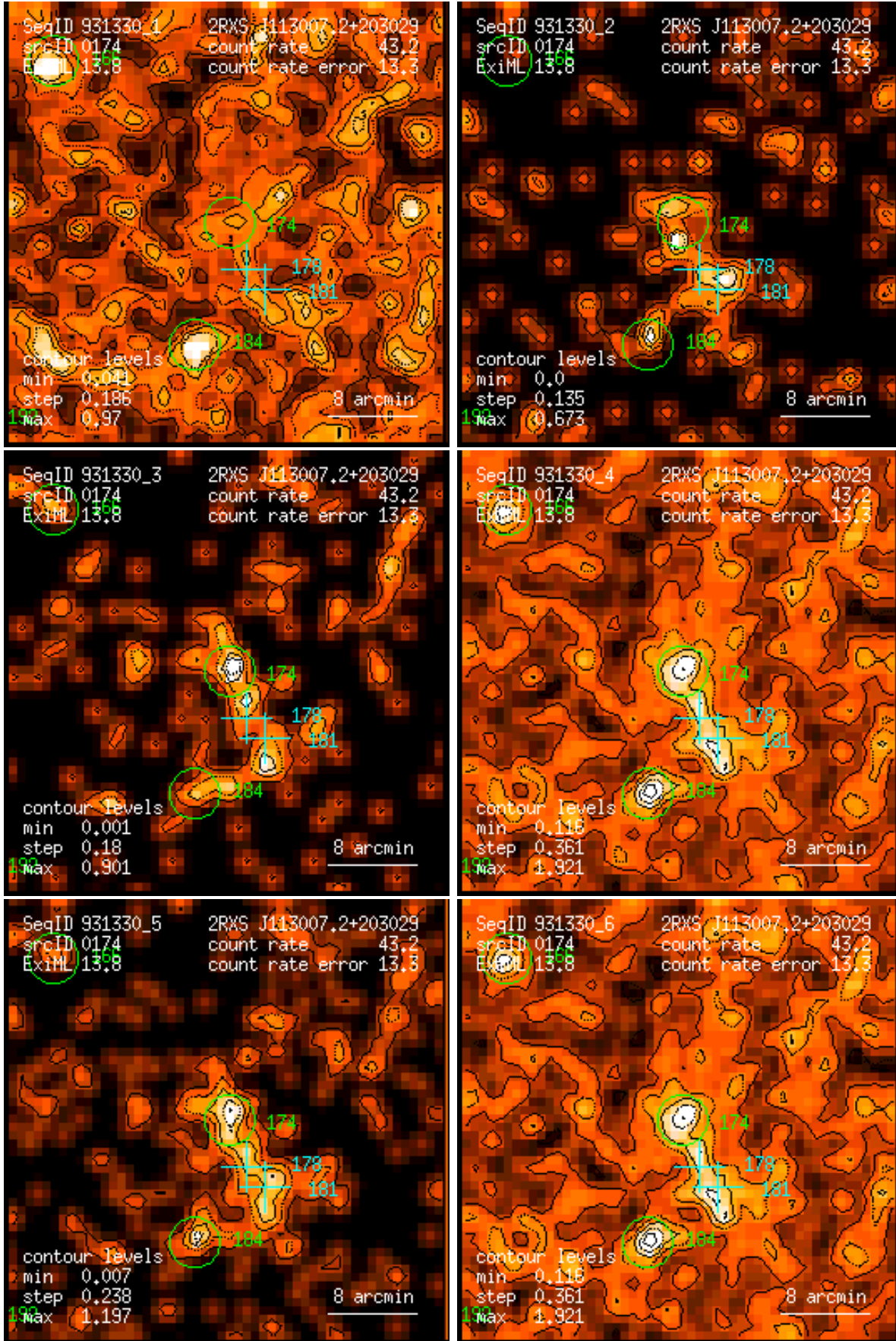
Figure 174: RASS 931330: detection 0174: band rate images, Gaussian filter: (1) PSPC channels 11 – 41, (2) 52 – 90, (3) 91 – 201, (4) 11 – 235, (5) 52 – 201, (6) 11 – 201. Broad band rates in counts/ks. Band rate contour levels in counts/ks/arcmin 2 .
