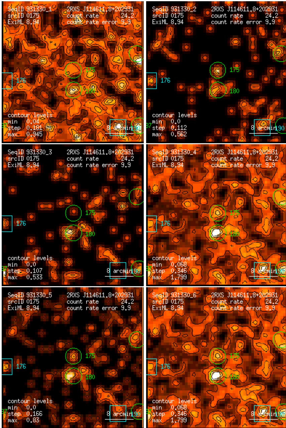
Figure 175: RASS 931330: detection 0175: band rate images, Gaussian filter: (1) PSPC channels 11 – 41, (2) 52 – 90, (3) 91 – 201, (4) 11 – 235, (5) 52 – 201, (6) 11 – 201. Broad band rates in counts/ks. Band rate contour levels in counts/ks/arcmin 2 .
