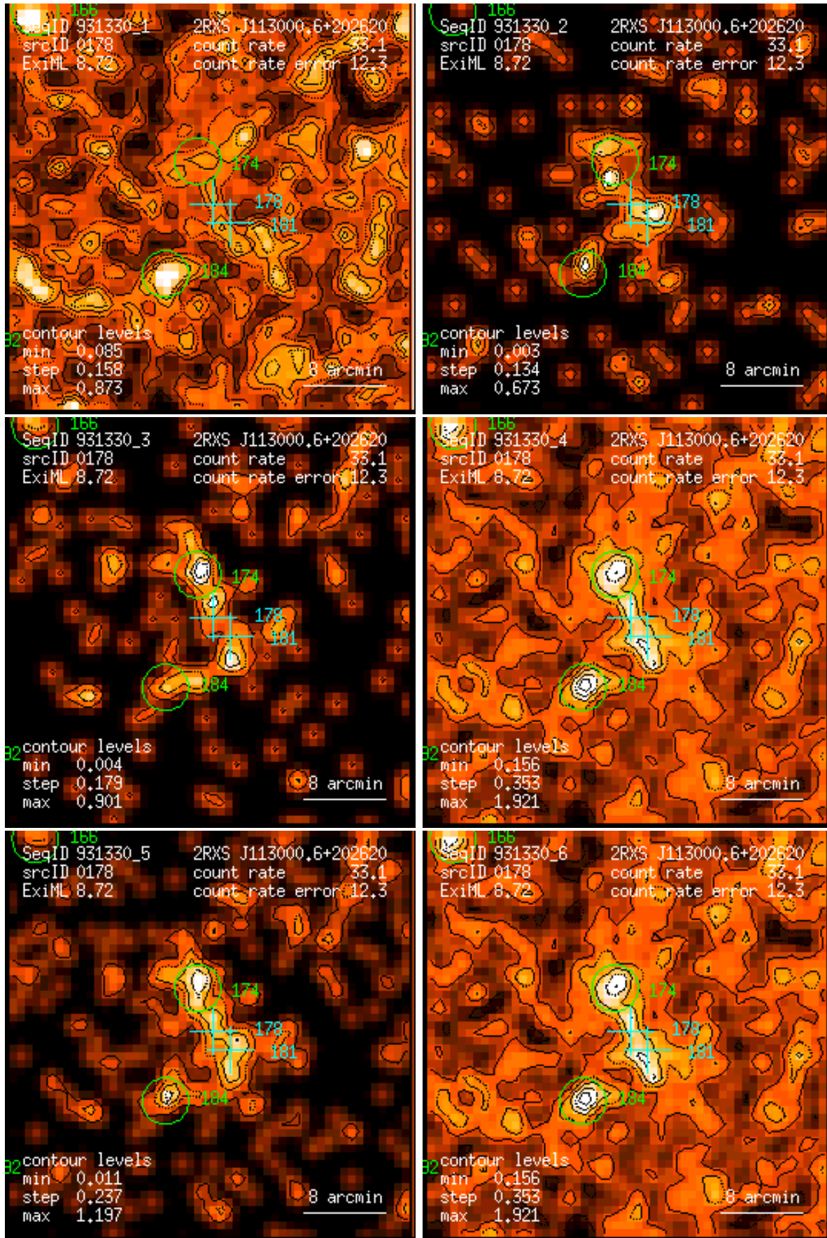
Figure 178: RASS 931330: detection 0178: band rate images, Gaussian filter: (1) PSPC channels 11 – 41, (2) 52 – 90, (3) 91 – 201, (4) 11 – 235, (5) 52 – 201, (6) 11 – 201. Broad band rates in counts/ks. Band rate contour levels in counts/ks/arcmin 2 .
