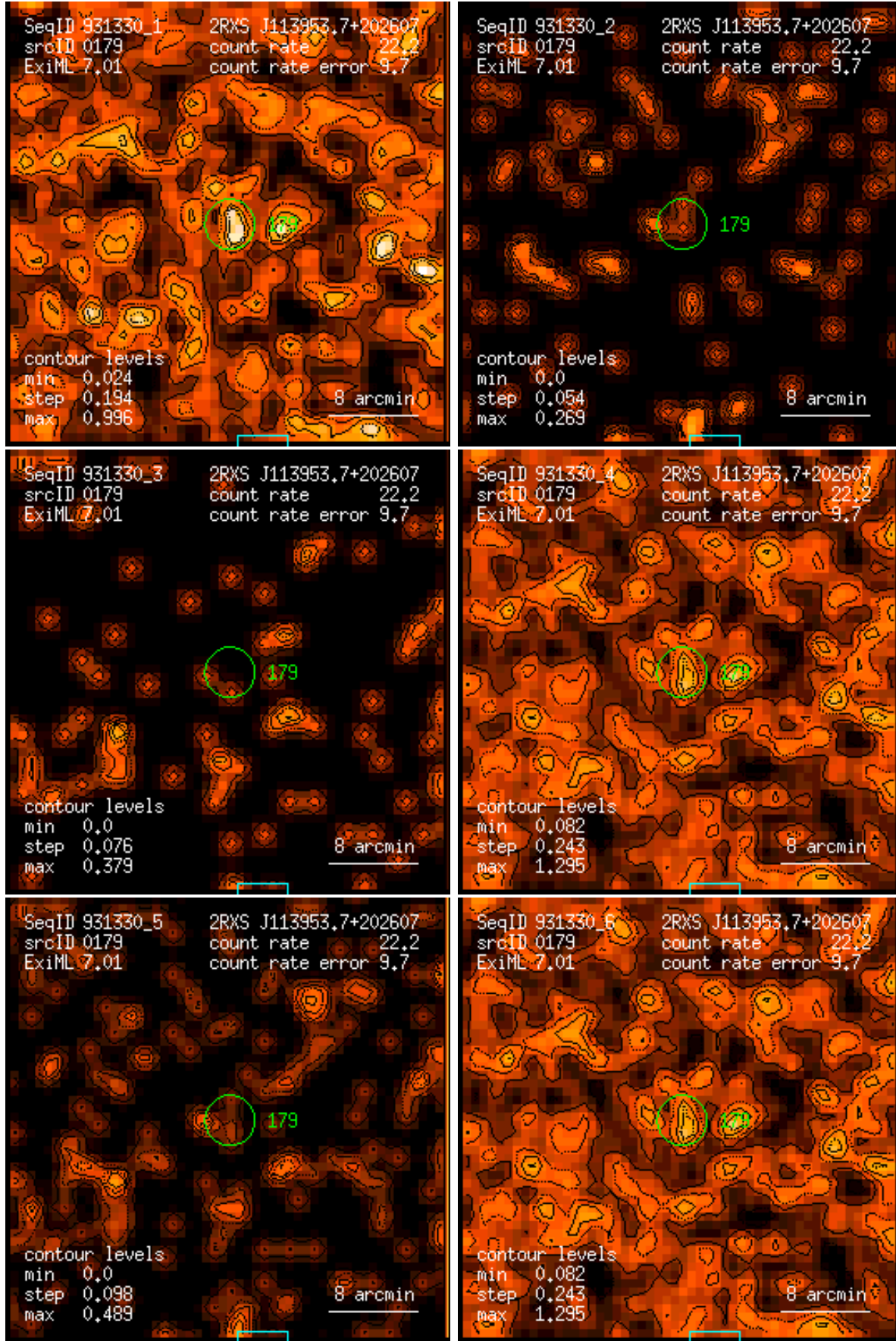
Figure 179: RASS 931330: detection 0179: band rate images, Gaussian filter: (1) PSPC channels 11 – 41, (2) 52 – 90, (3) 91 – 201, (4) 11 – 235, (5) 52 – 201, (6) 11 – 201. Broad band rates in counts/ks. Band rate contour levels in counts/ks/arcmin 2 .
