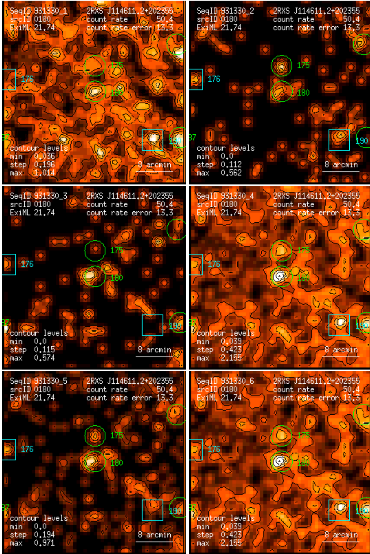
Figure 180: RASS 931330: detection 0180: band rate images, Gaussian filter: (1) PSPC channels 11 – 41, (2) 52 – 90, (3) 91 – 201, (4) 11 – 235, (5) 52 – 201, (6) 11 – 201. Broad band rates in counts/ks. Band rate contour levels in counts/ks/arcmin 2 .
