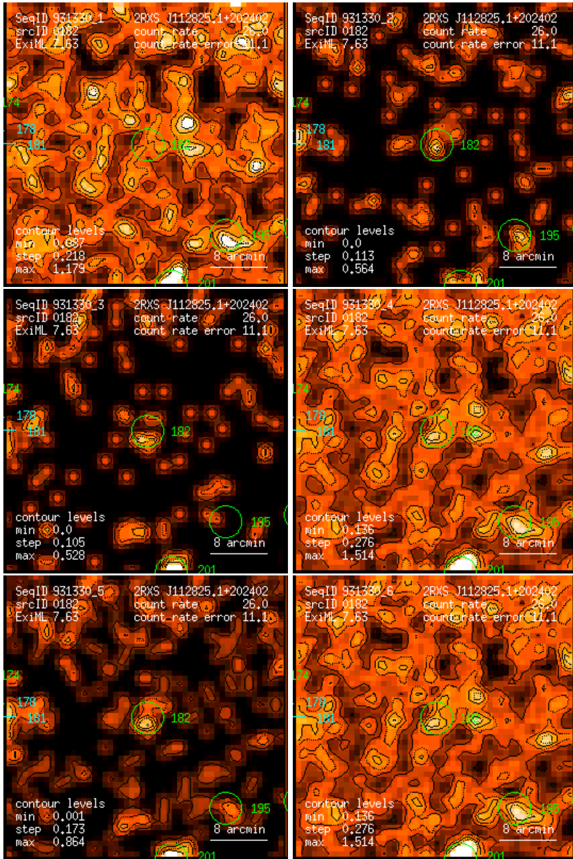
Figure 182: RASS 931330: detection 0182: band rate images, Gaussian filter: (1) PSPC channels 11 – 41, (2) 52 – 90, (3) 91 – 201, (4) 11 – 235, (5) 52 – 201, (6) 11 – 201. Broad band rates in counts/ks. Band rate contour levels in counts/ks/arcmin 2 .
