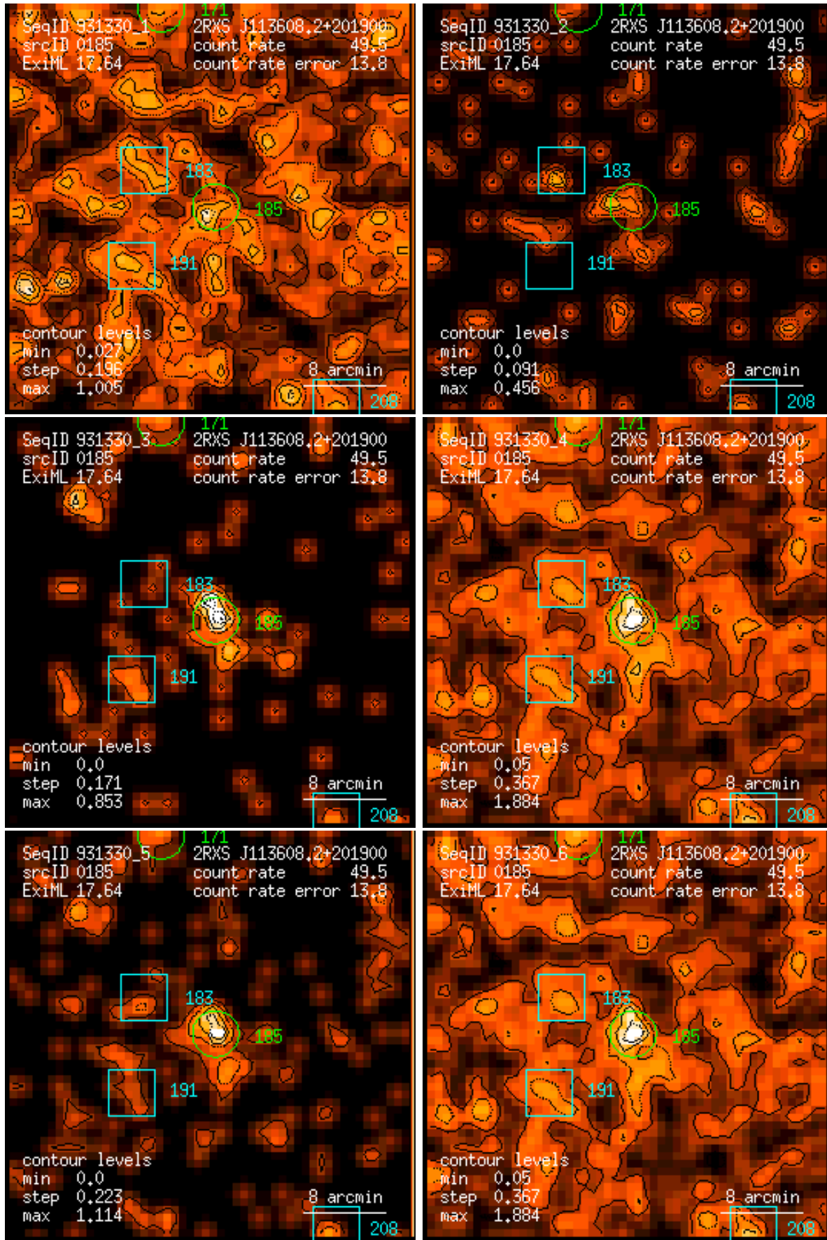
Figure 185: RASS 931330: detection 0185: band rate images, Gaussian filter: (1) PSPC channels 11 – 41, (2) 52 – 90, (3) 91 – 201, (4) 11 – 235, (5) 52 – 201, (6) 11 – 201. Broad band rates in counts/ks. Band rate contour levels in counts/ks/arcmin 2 .
